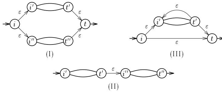
Fig. 4.2. Normalized extended automata recognizing the regular expressions \mathbf{u} + \mathbf{v} (I), \mathbf{u} \cdot \mathbf{v} (II), and \mathbf{u}^* (III), obtained from normalized extended automata (Q', i', \{t'\}, E') and (Q'', i'', \{t''\}, E'') recognizing respectively the regular expressions \mathbf{u} and \mathbf{v} .
