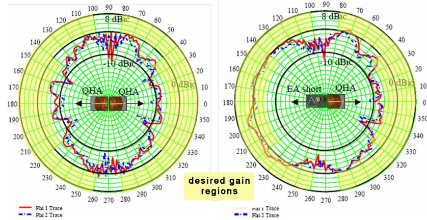
Figure 3. Measured patterns on ST-5 mock-up of two QHAs and a ST5-104.33 with a QHA. \Phi_1 = 0 deg., \Phi_2 = 90 deg.
