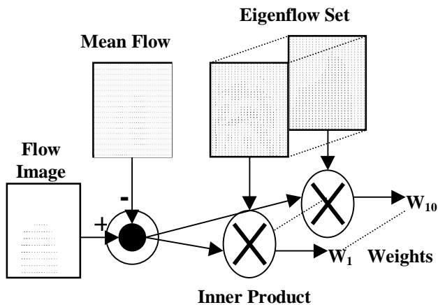
Figure 7. Horizontal weight vector computation.
