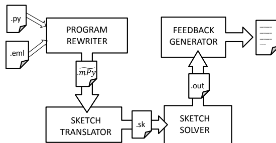
Figure 3. The architecture of our feedback generation tool.
