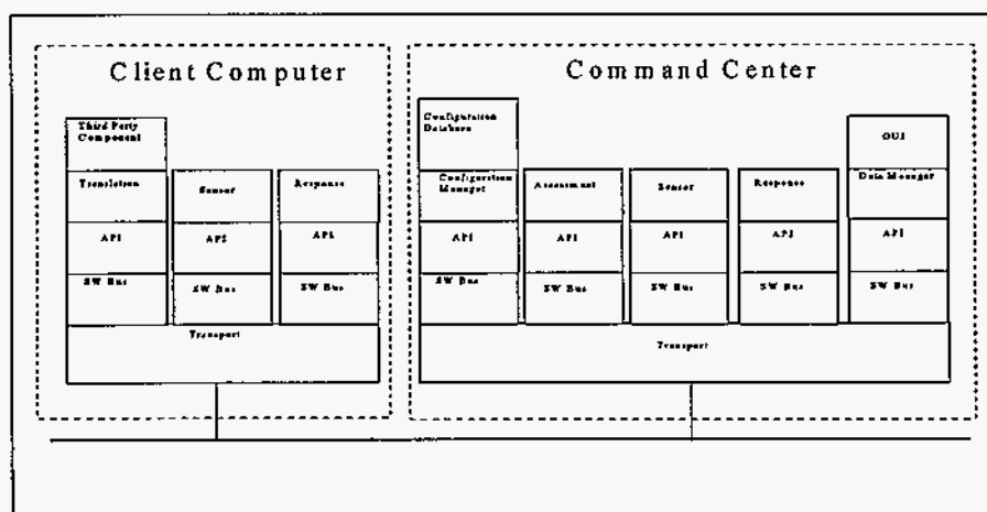
Figure 4. Alarm System Architecture
