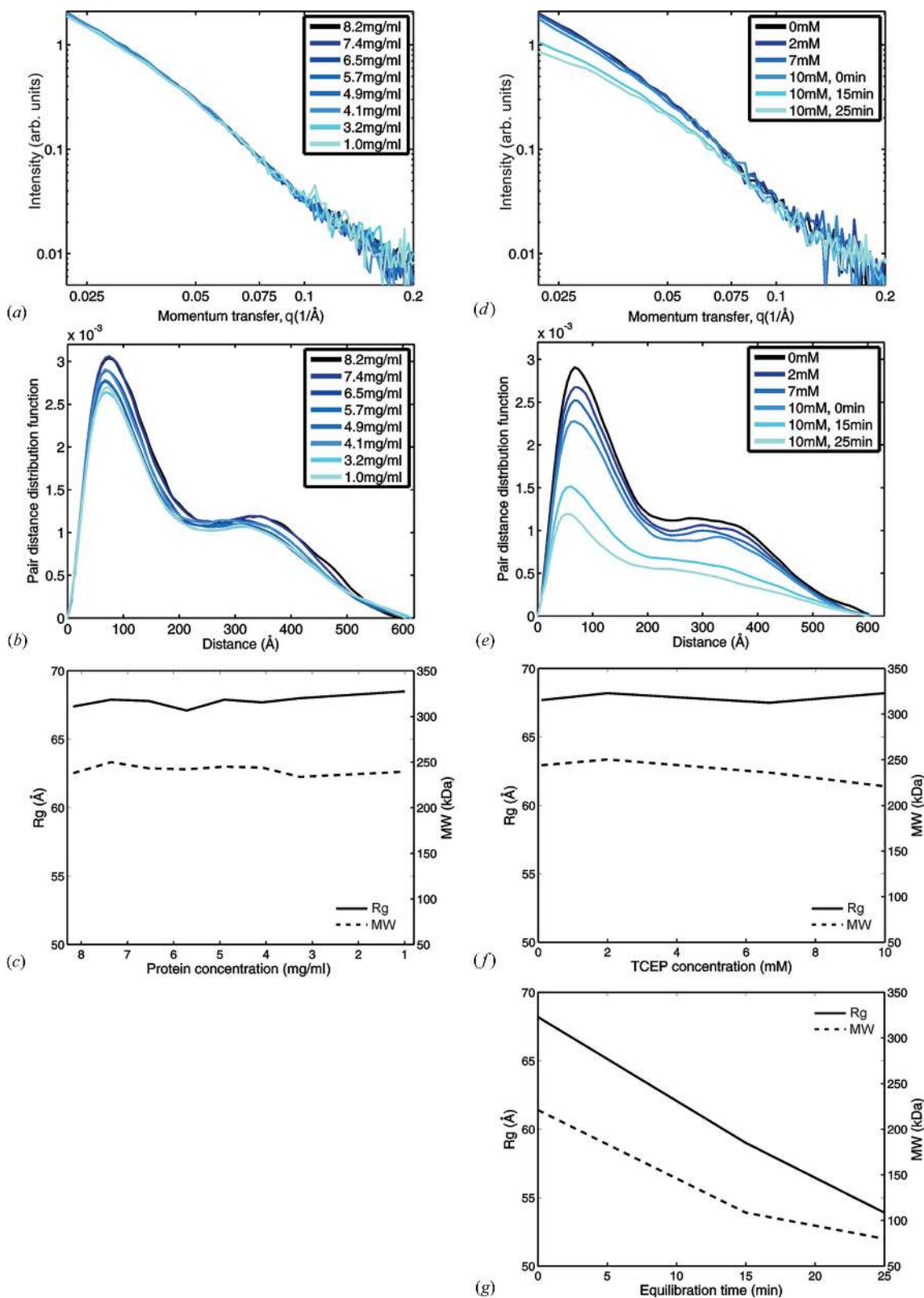
Figure 6 Exploration of the structural space of N2, starting from non-reduced conditions. The left-hand column shows data for N2 dilution with non-reducing buffer: (a) background-subtracted SAXS data normalized to protein concentration, (b) the corresponding pair distance distribution functions, p(r) , and (c) estimated radius of gyration ( R_g ) and molecular weight (MW). The right-hand column shows data for N2 titration with the reducing agent TCEP (0–10 mM): (d) background-subtracted SAXS data normalized to protein concentration, (e) the corresponding p(r) functions, (f) estimated R_g and MW as a function of TCEP concentration, and (g) estimated R_g and MW for N2 diluted in 10 mM TCEP after 0–25 min equilibration. The raw data and p(r) plots for the equilibrated solutions are shown in panels (d) and (e) using lighter blue colours.
