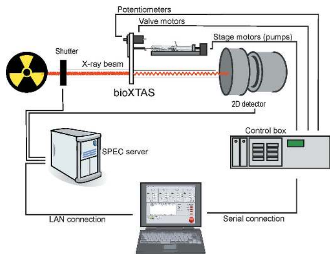
Figure 2 Schematic diagram of the automation setup.
