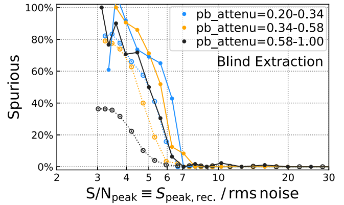
Figure 9. Spurious fraction for three bins of pb\_attenu : (0.2–0.34], (0.34–0.58] and (0.58–1.0], which are equally distributed in logarithm. The solid and dashed lines represent differential and cumulative curves, respectively (see Figure 8 caption). We caution that the trend seen here suffers from a strong bias in statistics, because the lowest pb\_attenu (farthest away from phase center) bin has only about 62 S/N_{\text{peak}} > 5 detections in original images and 27 in inverted images, while the numbers are 10 times larger in the innermost bin with pb\_attenu \sim 0.58 –1.0 (although they are equal in area).
