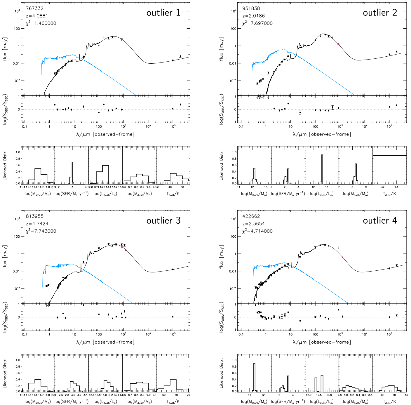
Figure 36. Example of SEDs for sources 1, 2, 3, and 4 listed in Figure 24 that exhibit strong mid-IR AGN emission and show disagreement in the stellar masses between this work and Delvecchio et al. (2017). See discussion of each source in Section 4.6. For each source, the best-fit full SED (black line) and unattenuated stellar SED (cyan line), as well as the photometric data points, are shown in the top, large subpanel. The ALMA data point from this work is highlighted in red. Optical to near-IR K -band data are from the “COSMOS2015” catalog (Laigle et al. 2016) with 3'' aperture photometry; near-IR IRAC to millimeter and radio data are from the “super-deblended” FIR/millimeter catalog (Jin et al. 2018). The SED fitting residuals at each band ( \log_{10} S_{\text{OBS}}/S_{\text{SED}} ) are shown in each middle subpanel. The probability distribution histograms of each fitted physical parameter ( \log_{10} M_* , \log_{10} SFR, IR luminosity \log_{10} L_{\text{dust}} , dust mass \log_{10} M_{\text{dust}} , and dust temperature T_{\text{dust}} ) are shown in the subpanels at the bottom.
