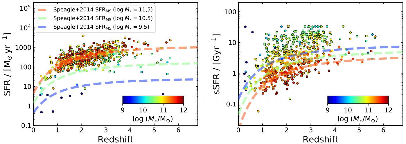
Figure 25. Distribution of SFR (left) and sSFR (right) vs. redshift. Empirical evolution curves of the star-forming MS at different stellar masses ( \log_{10}(M_*/M_\odot) = 9.5, 10.5, and 11.5, respectively) are shown as blue, green, and red dashed lines, which are computed as a function of redshift and M_* following Speagle et al. (2014) (the #49 model in their Table 7). The color bar indicates \log_{10} M_* in both panels.
