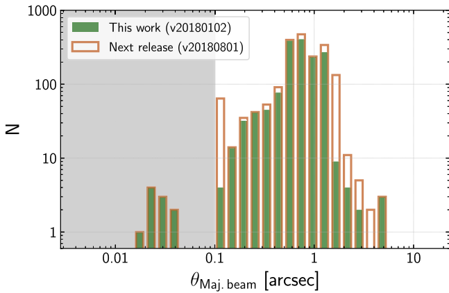
Figure 5. Beam size distributions of two versions of A 3 COSMOS data sets. The beam size is defined as the FWHM along the major axis of ALMA data’s synthesized beam ( \theta_{\text{Maj,beam}} ) after the interferometric “cleaning” process. The gray shaded area indicates \theta_{\text{Maj,beam}} < 0.1'' , for which data were discarded owing to too high spatial resolution as discussed at the end of Section 2.1.
