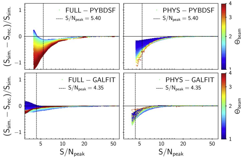
Figure 12. Flux bias (as defined in Equation (3)) vs. the measured S/N_{\text{peak}} (as defined in Equation (1)) statistics for PYBDSF (top panels) and GALFIT (bottom panels) photometry, each based on our two types of MC simulations (left panels are “FULL” simulation, and right panels are “PHYS” simulation; see the label in each panel). Color represents the geometric mean source-to-beam size ratio ( \Theta_{\text{beam}} , as defined in Equation (2) in Section 2.2) and is the same in all four panels. Vertical lines are our S/N_{\text{peak}} thresholds for the sample selection in Section 4.1.
