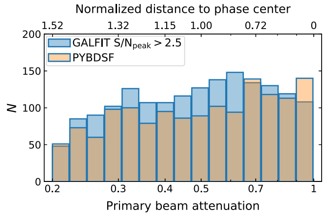
Figure 10. Radial distribution of spurious detections for the PYBDSF-based blind source extraction (orange) and GALFIT-based prior source fitting (blue). The bottom x-axis is the PBA, pb\_attenu , and the top axis is the normalized distance to the phase center, \text{dist.}/(0.5 \times pb) , where \text{dist.} is the spatial distance to the phase center and pb is the FWHM of the primary beam. The histogram bins are equally distributed in \ln(pb\_attenu) (so that the areas of each bin normalized by the primary beam area are equal).
