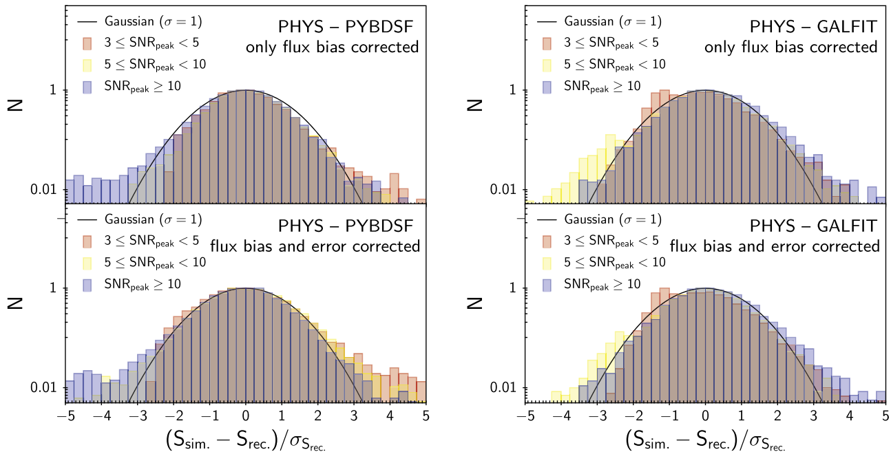
Figure 33. Left panels are based on the “PHYS” simulation with PYBDSF photometry, and right panels are based on the “PHYS” simulation with GALFIT photometry. In each left/right panel, the top panel is the histogram of (S_{\text{sim.}} - S_{\text{rec.}}^{\text{corr.}})/\sigma_{S_{\text{rec.}}^{\text{Condon1997}}} , where S_{\text{rec.}}^{\text{corr.}} is the measured total flux after flux bias correction (Section 3.1.1) and \sigma_{S_{\text{rec.}}^{\text{Condon1997}}} is the error in total flux shipped with PYBDSF based on Condon (1997). The bottom panel is the histogram of (S_{\text{sim.}} - S_{\text{rec.}}^{\text{corr.}})/\sigma_{S_{\text{rec.}}^{\text{corr.}}} , where \sigma_{S_{\text{rec.}}^{\text{corr.}}} is the simulation-based error in total flux (Section 3.1.3). A 1D Gaussian with mean = 0 and \sigma = 1 is overlaid in each panel.
