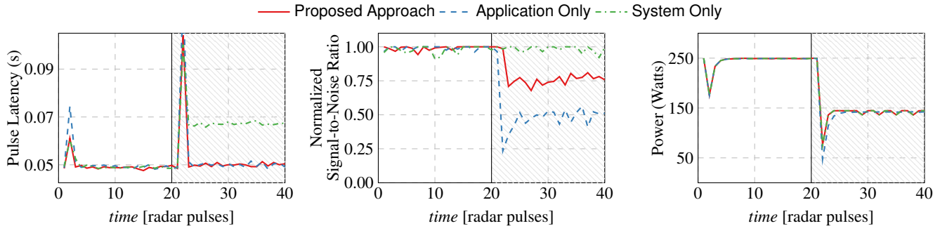
Figure 3: Radar results: performance, energy consumption and accuracy over time.
