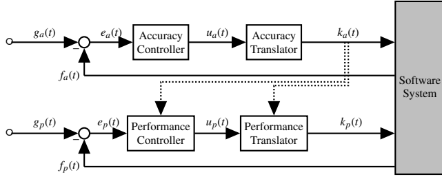
Figure 1: Block diagram for controlling accuracy and performance.
