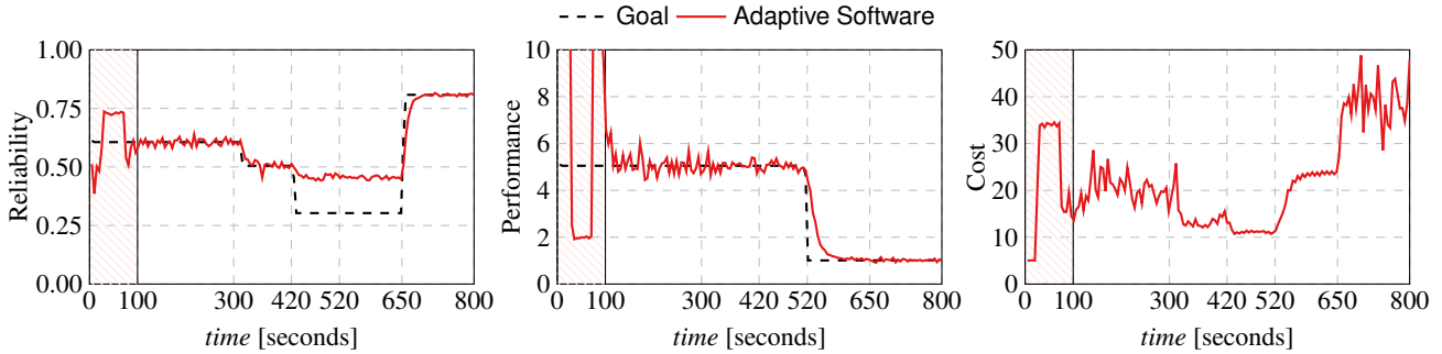
Figure 4: Service Dynamic Binding results: reliability, performance and cost over time.
