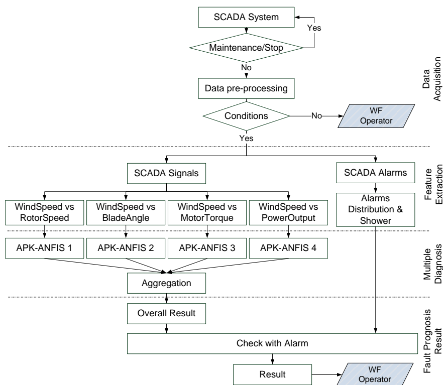
Figure 5: The proposed prognosis procedure
