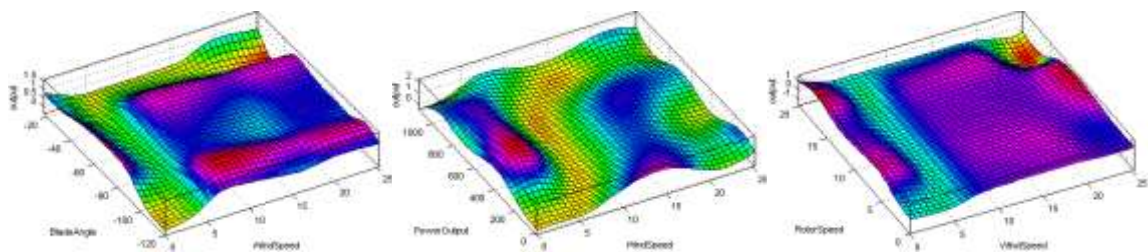
Figure 10: Output surfaces generated from the trained APK-ANFIS models
