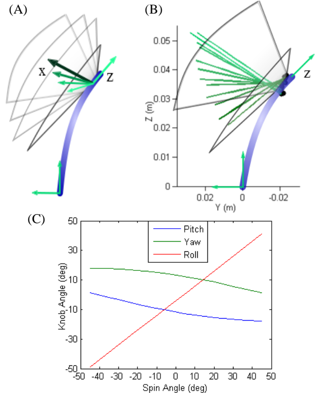
Figure 7: (a) Simulation showing the catheter spinning about its own axis, (b) spinning test results with blue lines to represent the imaging plane axis rotation, (c) joint angles required to actuate motion
