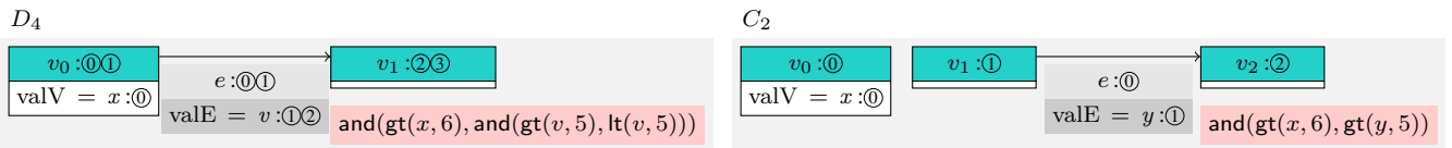
Figure 12: An example of an application of the shift -operation.
