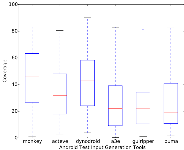
Fig. 1. Variance of coverage achieved across 10 runs.
