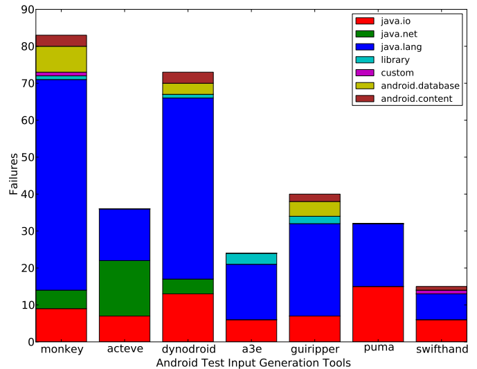
Fig. 3. Distribution of the failures triggered by the tools.
