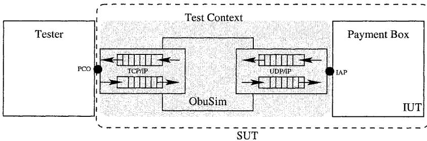
Figure 3. Test architecture
