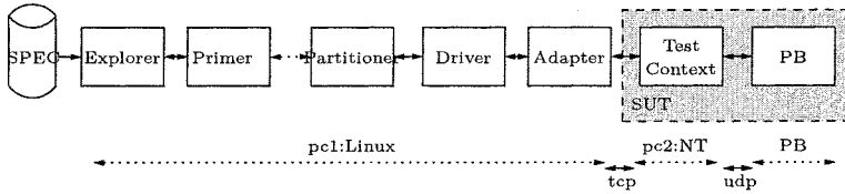
Figure 2. TORX tool architecture
