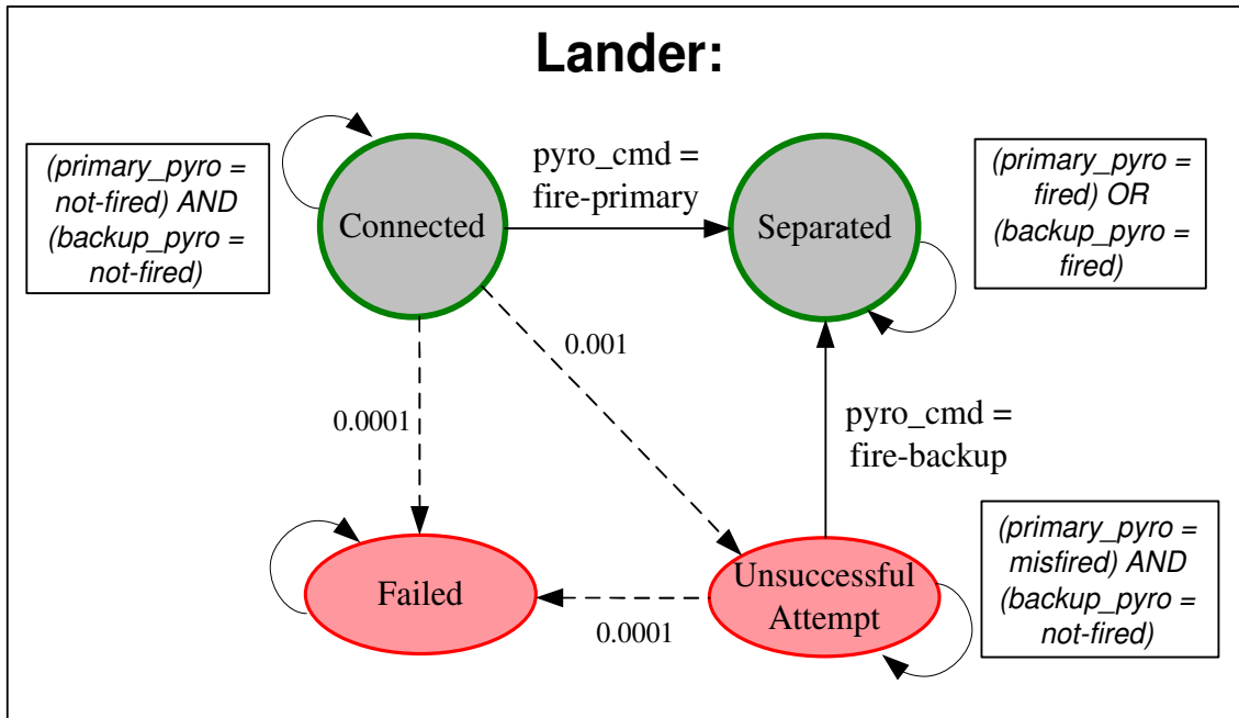
Figure 5-8: The Lander Component.
