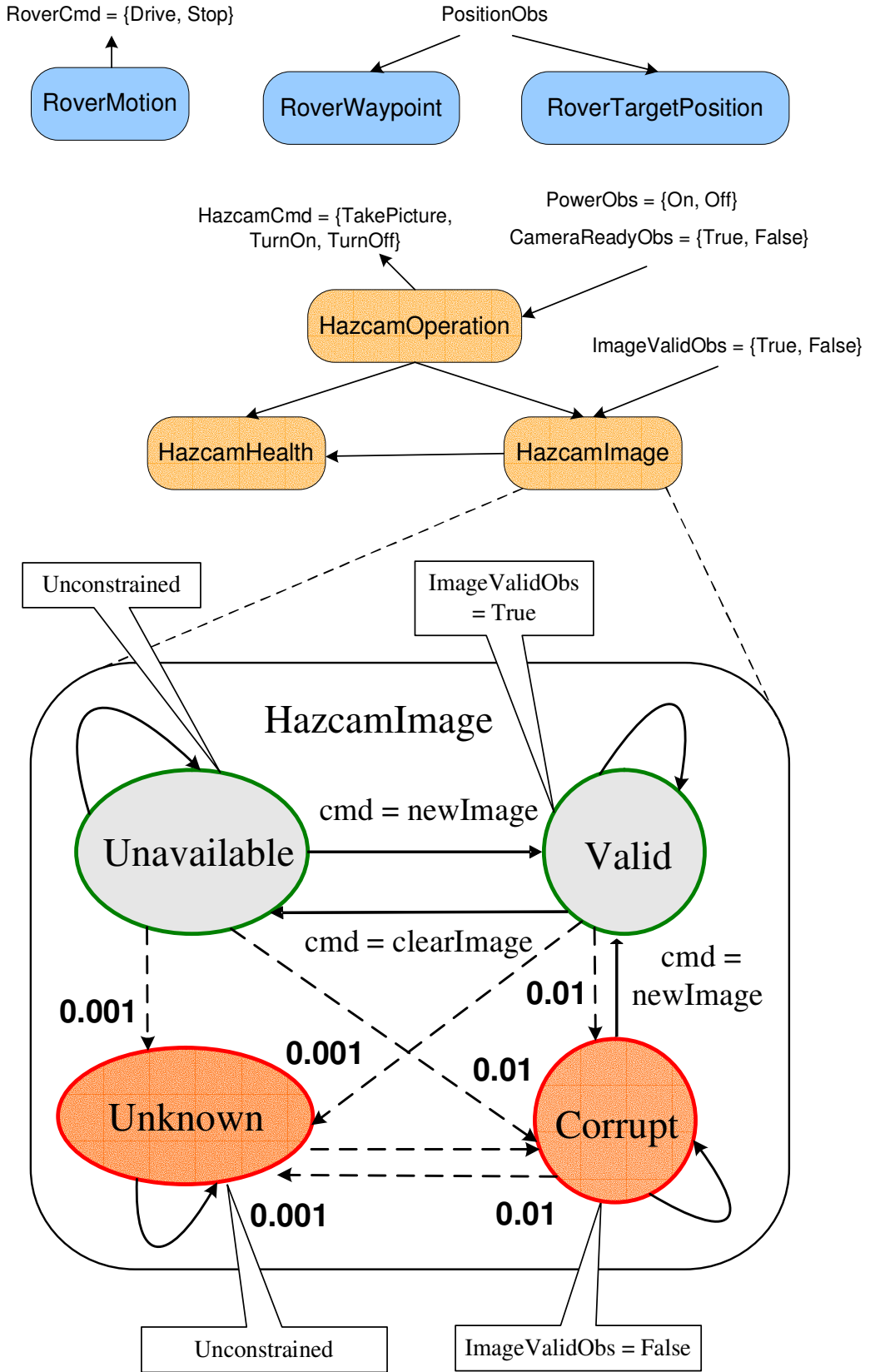
Figure 3-3: The Plant Model for the Rover-Hazcam Scenario.
