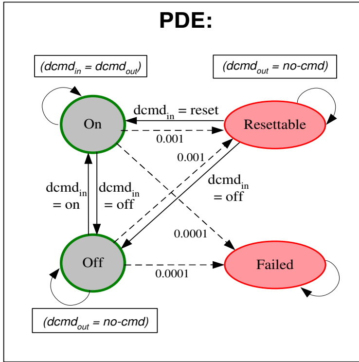
Figure 5-10: The PDE Component.
