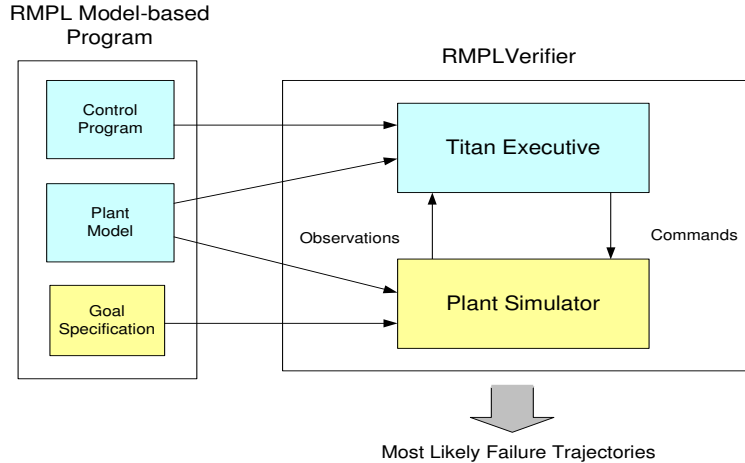
Figure 4-2: A High-level View of the Algorithm.
