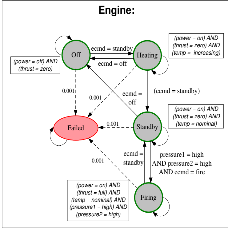
Figure 5-6: The Engine Component.
