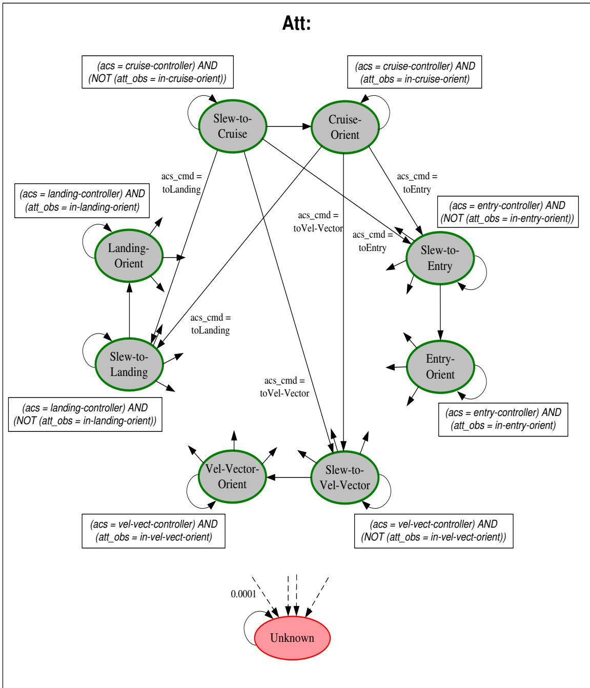
Figure 5-5: The Att Component.
