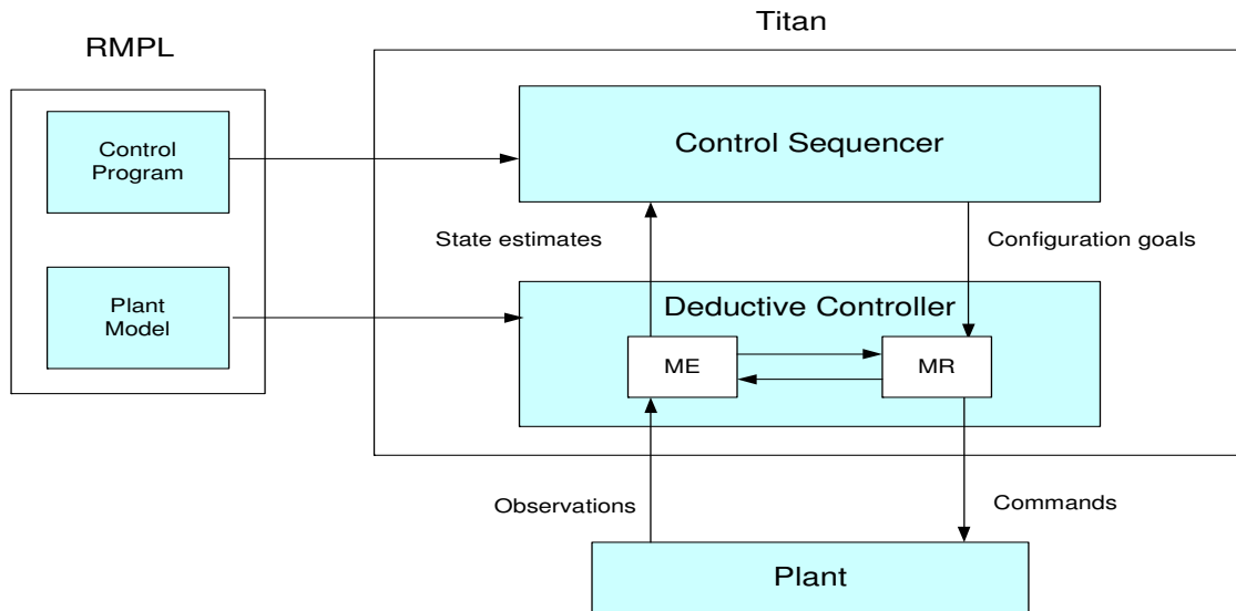
Figure 3-4: The Architecture of the Titan Model-based Executive.
