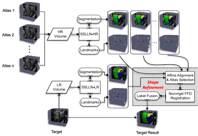
Fig. 2. Pipeline for automatic bi-ventricular segmentation of low- and high-resolution volumetric images. The pipeline includes segmentation, landmark localization and atlas propagation. It is capable of producing accurate, high-resolution and anatomically smooth bi-ventricular models, despite existing artifacts in input CMR volumes.
