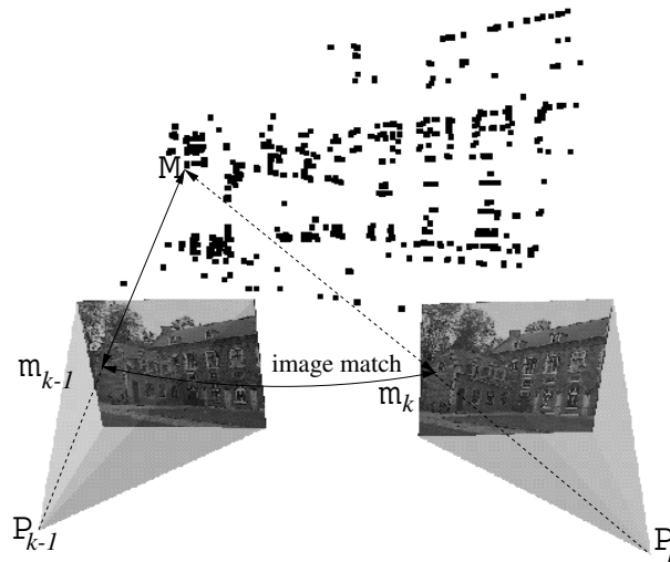
Figure 2: Image matches ( m_{k-1} , m_k ) are found as described before. Since the image points, m_{k-1} , relate to object points, M_k , the pose for view k can be computed from the inferred matches ( M , m_k ).
