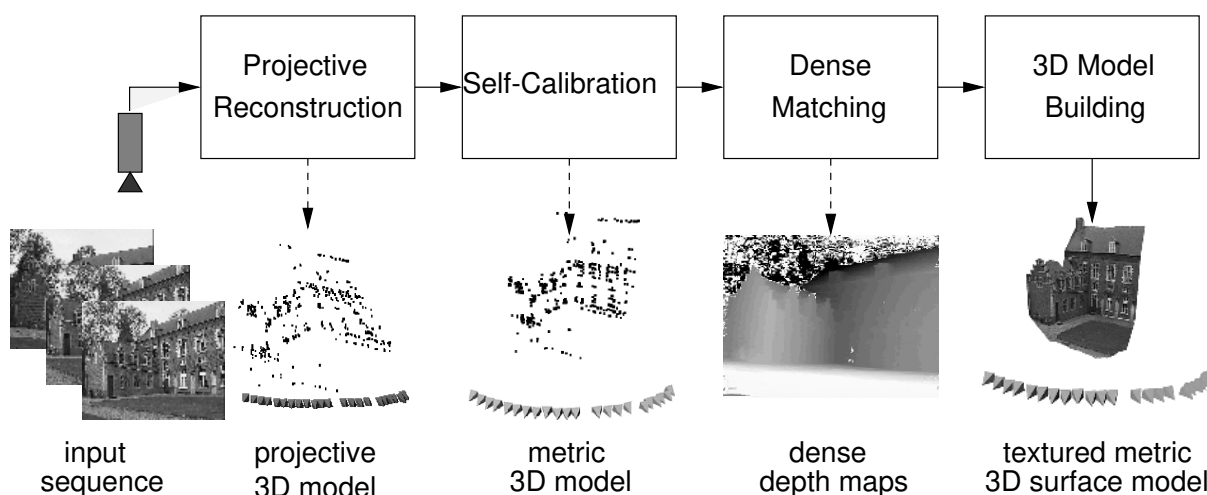
Figure 1: Overview of the system (the cameras are represented by little pyramids, the results of the dense matching are accumulated in dense depth maps where light means close and dark means far).
