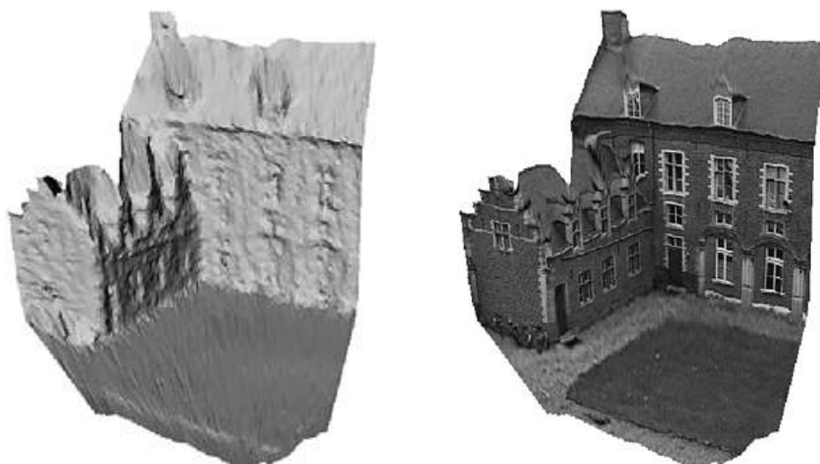
Figure 6: 3D surface model obtained automatically from an uncalibrated image sequence, shaded (left), textured (right).
