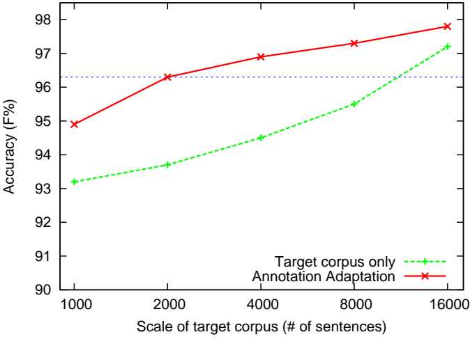
Figure 13 Performance of annotation adaptation with varying-size target corpora for Chinese word segmentation.
