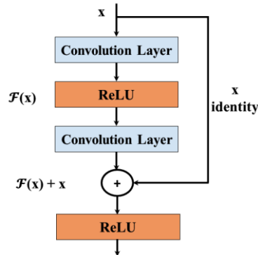
Fig. 1. Building Block of ResNet
