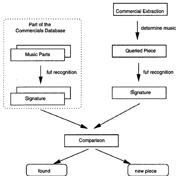
Figure 6: Retrieval of commercials
