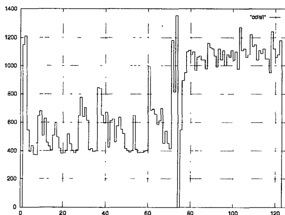
Figure 4: Distance diagram of file youtook.au
