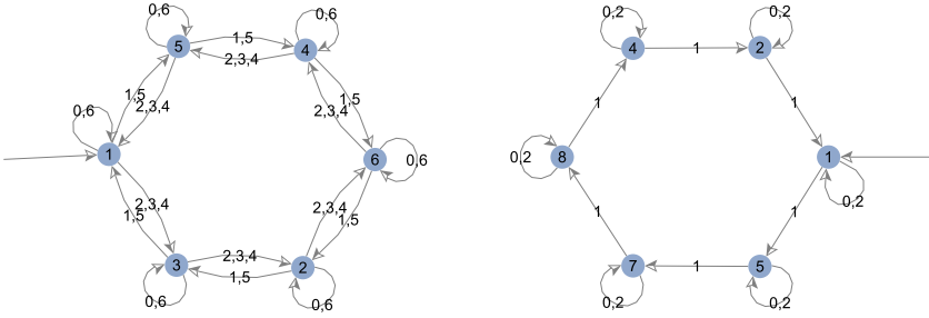
FIGURE 3.6. Automata that compute Apéry numbers modulo 7 (left) and 9 (right).
