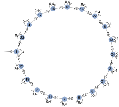
FIGURE 3.7. A subautomaton computing certain Apéry numbers modulo 25.
