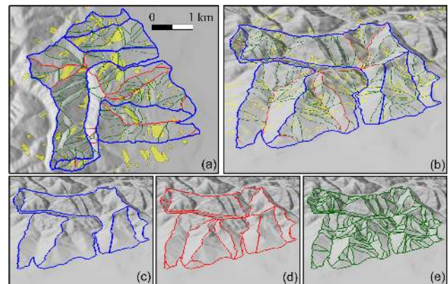
Figure 7. Example of subdivisions into SUs for a portion of the study area. Legend: blue, red, and green lines show boundaries of SUs of increasing density and corresponding decreasing average size. Yellow areas are landslides. The five maps show the same area in plan view (a) and in perspective view (b, c, d, e).
