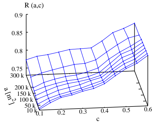
Figure 11. Values of the AUC_{ROC} calculated for LS maps estimated using SU partitions derived for different combination of the a and c user-defined modeling parameters.
