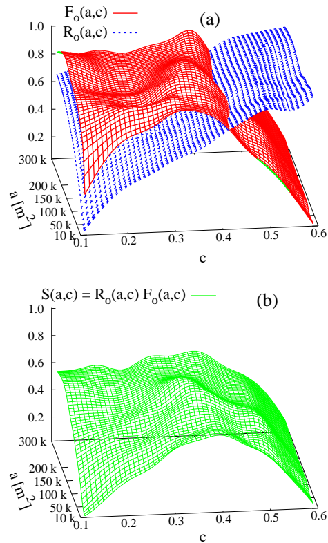
Figure 13. (a) R_o(a,c) (blue) and F_o(a,c) (red) functions, defined by Eqs. (9) and (10). (b) S_o(a,c) function defined by Eq. (11). The functions were interpolated on a denser mesh for improved visual representation.
