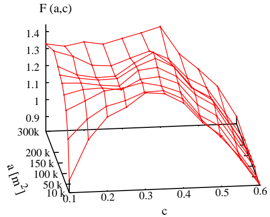
Figure 9. Segmentation objective function values (Eq. 3) calculated for 99 SU partitions obtained using different combinations of the a and c parameters.
