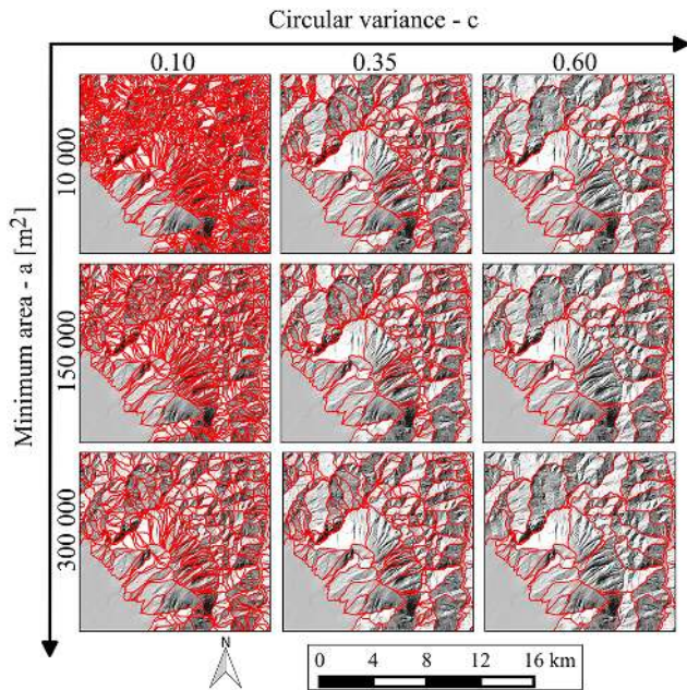
Figure 6. A group of 9 (out of 99) SU terrain subdivisions for a portion of the study area. The SUs were obtained changing the a and c parameters used by the r.slopeunit software. The maps are in the UTM zone 32, datum ED50 (EPSG:23032) reference system.
