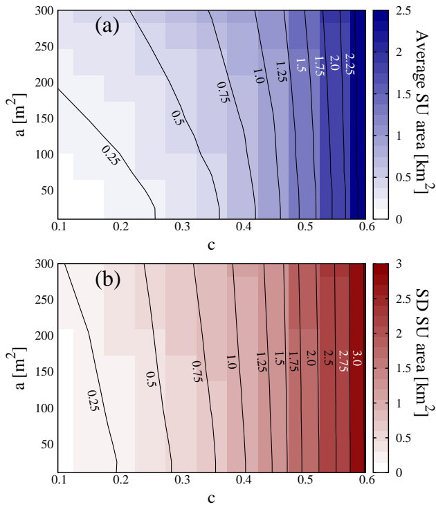
Figure 8. (a) Average and (b) standard deviation of the size of the SUs, for different combinations of a and c parameters. The minimum size of the SUs is fixed by the a parameter, and the maximum size of the SUs is independent of a .
