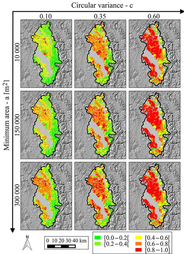
Figure 10. The group of 9 (out of 99) LS maps obtained with different SU partitions resulting from different combinations of the a and c parameters. The maps are in the UTM zone 32, datum ED50 (EPSG:23032) reference system.
