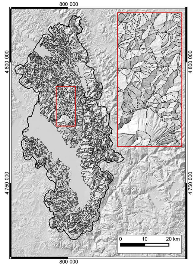
Figure 14. The SU subdivision corresponding to the best parameters selected by our optimization procedure. The values of the parameters are a = 150\,000\text{ m}^2 , a = 0.35 . The associated LS result is shown in Fig. 10, in the central box, corresponding to the optimal parameters values.
