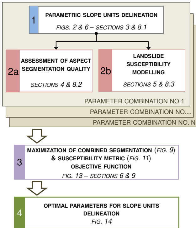
Figure 1. Logical framework for the proposed method for (1) the parametric delineation of SUs, (2a) the assessment of the quality of terrain aspect segmentation using of a proper segmentation objective function, (2b) the calculation and assessment of the quality of the LS modeling using a standard AUC_{ROC} metric, and (3) the definition and maximization of a combined objective function for (4) the determination of optimal parameters for the delineations of SUs best suited for LS modeling and zonation.
