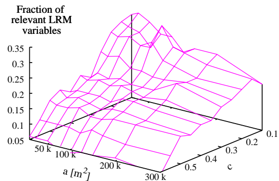
Figure 12. Percentage of relevant variables in the LRM used in this work to prepare the LS maps as a function of the a and c user-defined modeling parameters. Combination of a and c are the same used to prepare Fig. 11. Note that the direction of the axes is reversed with respect to Fig. 11.
