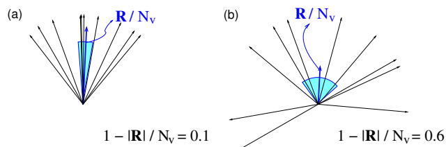
Figure 3. Graphical representation of the circular variance of terrain aspect, 1 - |\mathbf{R}|/N_v . Two groups of unit vectors are shown. The unit vectors represent the local direction of terrain aspect for each grid cell, resulting in circular variance (a) of 0.1 and (b) of 0.6. Unit vectors are perpendicular to the local topography, represented by the grid cell.
