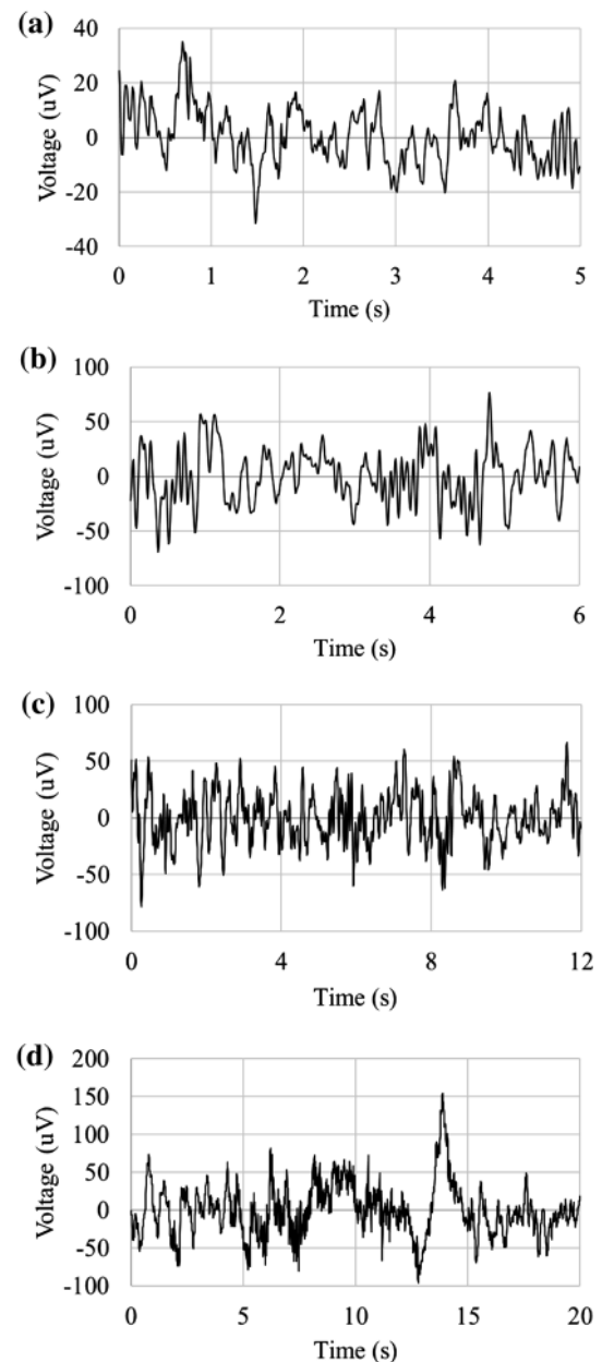
Fig. 1 Example of CAP phases, a B phase, b A1 subtype, c A2 subtype and d A3 subtype. From a to c , it is possible to detect the increase in rapid activities, and from a to any of the A phase subtypes ( b–d ), an increase in the signal amplitude variation occurs
