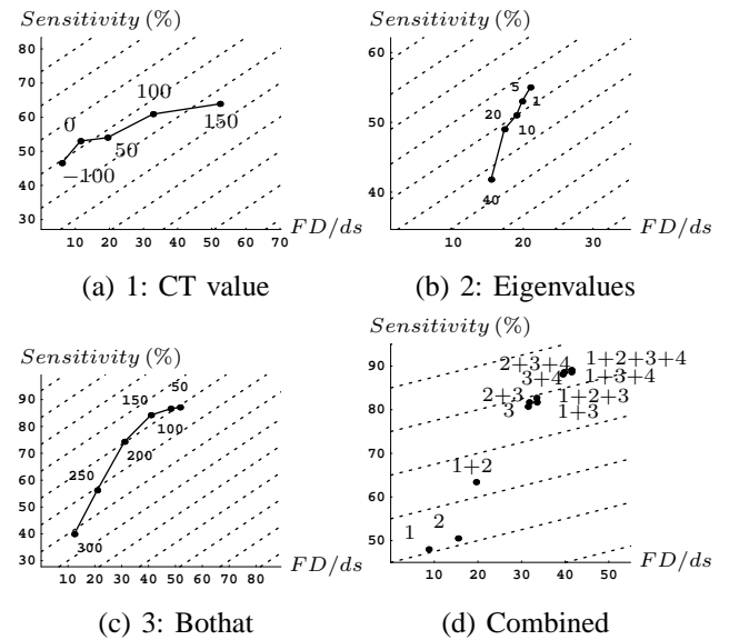
Fig. 3. (a-c) FROC for the thresholds of three intensity-based detectors and (d) a combination of the four detectors based on 1: CT value, 2: eigenvalues, 3: bothat and 4: vessel tracking. Thresholds of 0 HU, 1 and 150 were chosen for intensity, eigenvalues and bothat respectively to minimize the cost. The dashed lines represent lines of equal costs. The figure shows that the most important detectors are bothat and vessel tracking (3+4).
