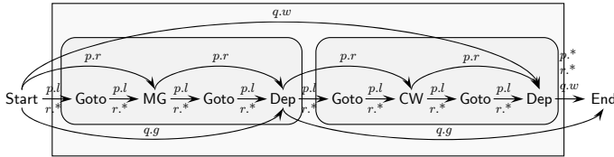
(c) The segment corresponding to collecting the requisite amount of wood ( q.w = 1 ) is extracted. Other literals entering this segment result in segments that are merged together with the q.g = 1 segment (merged goal condition not shown for clarity).
