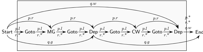
(a) The entire CAT is associated with the root task of collecting gold and wood. The root task terminates when the requisite amount of gold and wood have been collected.
