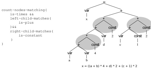
Figure 8. An example feature from the grammar in figure 7. In the right hand of the figure is a sample AST from the tiny language, showing the matching substructures. The feature thus evaluates to three.
