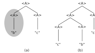
Figure 9. Mutation operator. In (a) a non-terminal is selected at random from an original parse tree. In (b) the non-terminal is replaced by a new random expansion of the same non-terminal.
