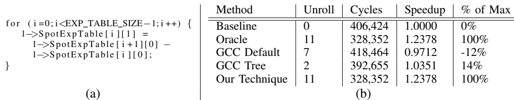
Figure 2. Loop from MediaBench (a) and speedups using various schemes (b). GCC’s default heuristic selects an unroll factor of 7 causing a slowdown. Using GCC features and machine learning, an unroll factor 2 is selected giving a small improvement. Our technique correctly determines 11 as the best unroll factor.
