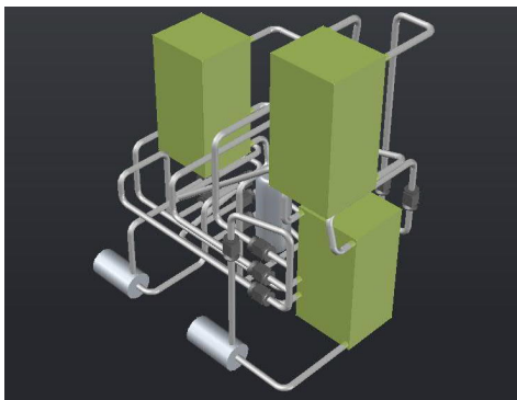
Fig. 6. 3D model of the HPP process
