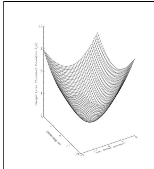
Figure 1: Surface plot of the standard deviation of the height error sampled along a kinematic GPS track over a mountainous SRTM cell [8]
