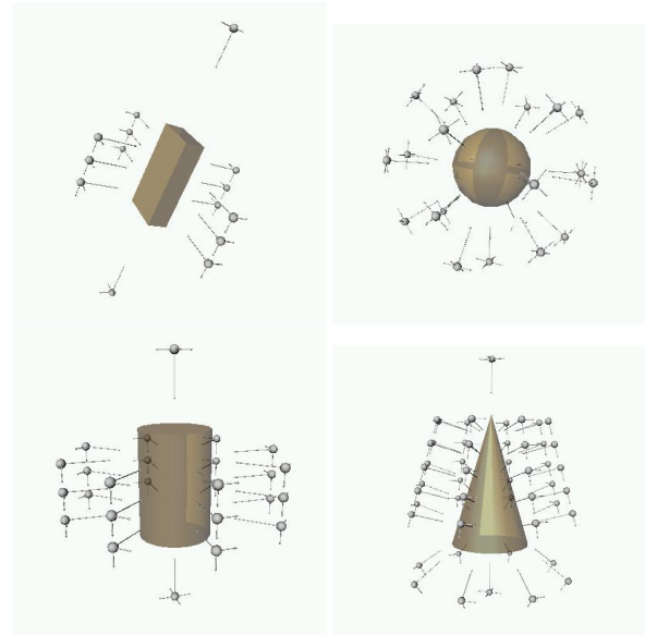
Figure 4: Examples for grasp generation on single primitives. The balls represent starting positions for the center of the palm. A long arrow shows the grasp approach direction (perpendicular to the palm face), and a short arrow shows the thumb direction (always perpendicular to the approach). In most grasp locations, two or more grasp possibilities are shown, each with a different thumb direction.
