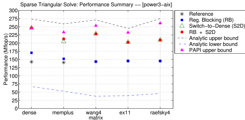
Figure 10: Performance summary (IBM Power3) : Performance (Mflop/s) of our SpTS implementations relative to various performance bounds (see Section 3.2). Register blocking evidently does not yield any significant performance improvements. The switch-to-dense optimization, however, tightens the performance gap. Note that two matrices have been omitted since they fit approximately within the large (8 MB) L2 cache.
