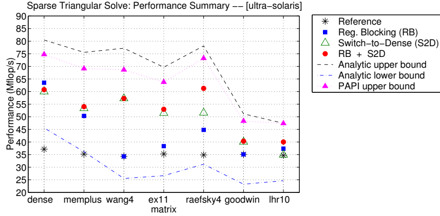
Figure 8: Performance summary (Sun Ultra 2i) : Performance (Mflop/s) shown for the seven items listed in Section 3.2. The best codes achieve 75–85% of the performance upper bound.
