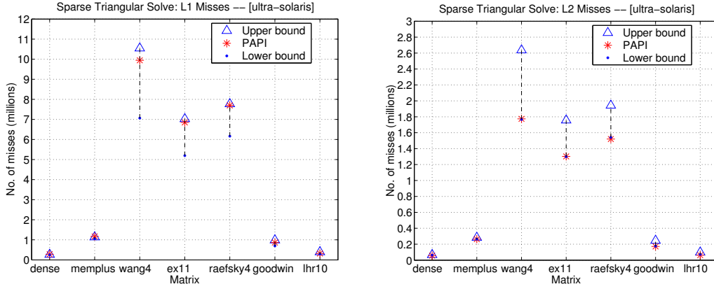
Figure 5: Miss model validation (Sun Ultra 2i) : Our upper and lower bounds on L1 and L2 cache misses compared to PAPI measurements. The bounds match the data well. The true L2 misses match the lower bound well in the larger (L2) cache, suggesting the vector sizes are small enough that conflict misses play a relatively minor role.
