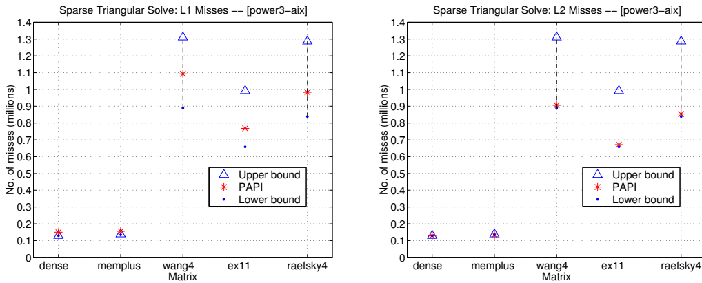
Figure 7: Miss model validation (IBM Power3) : Our upper and lower bounds on L1 and L2 cache misses compared to PAPI measurements. Note that two matrices have been omitted since they fit approximately within the large (8 MB) L2 cache.
