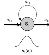
Figure 1: 1-state HMM. The one state HMM is a special 1-state model for the boundaries when the transition probabilities a_{11} = 0 and a_{12} = 1 .
