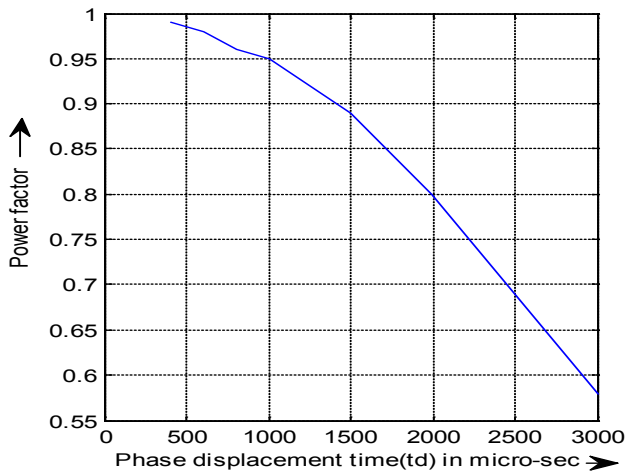
Figure 13 : Phase displacement time verses power factor
