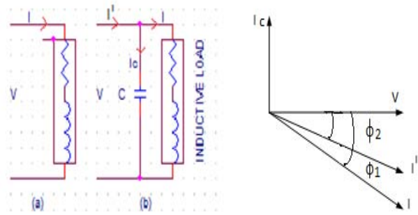
Figure 1 : Power factor improvement circuit and phasor diagram
