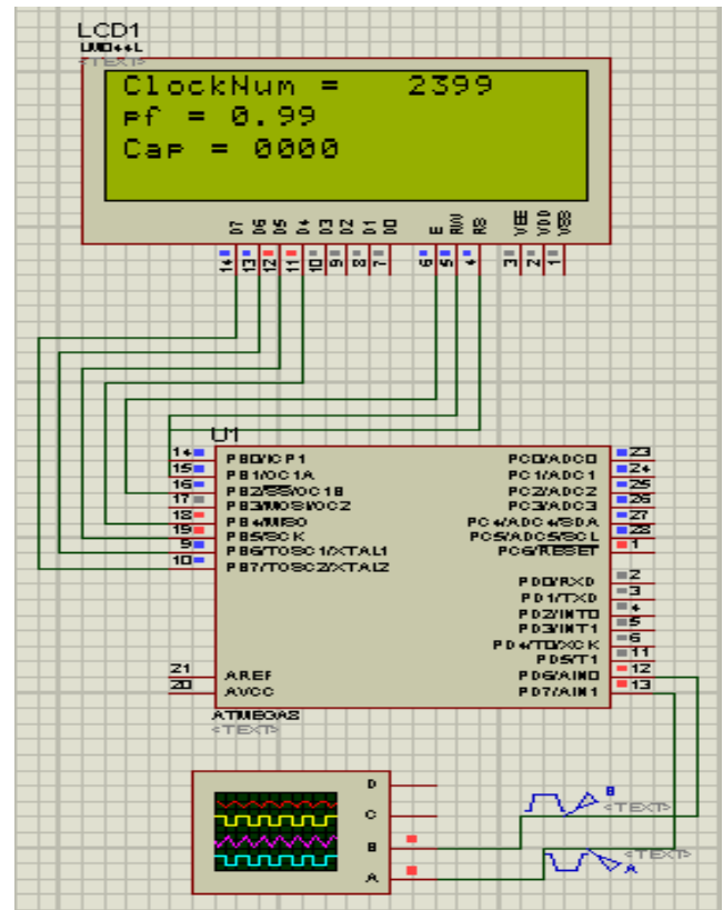
Figure 12 : Simulation Mode2
