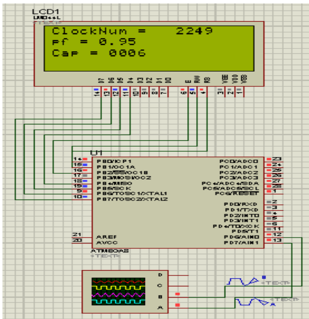
Figure 8 : Simulation Mode1
