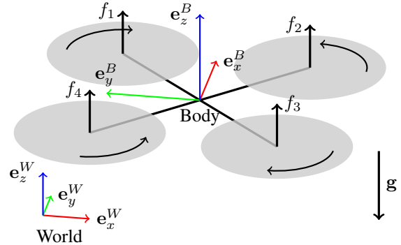
Fig. 3: Quadrotor with coordinate system and rotor forces.
