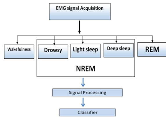
Fig. 1. Electromyogram
