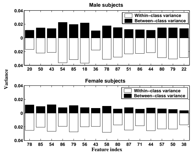
Figure 1: Feature assessment based on the ratio between the between-class variance ( \sigma_b^2 ) and the within-class variance ( \sigma_w^2 ) for each gender.
