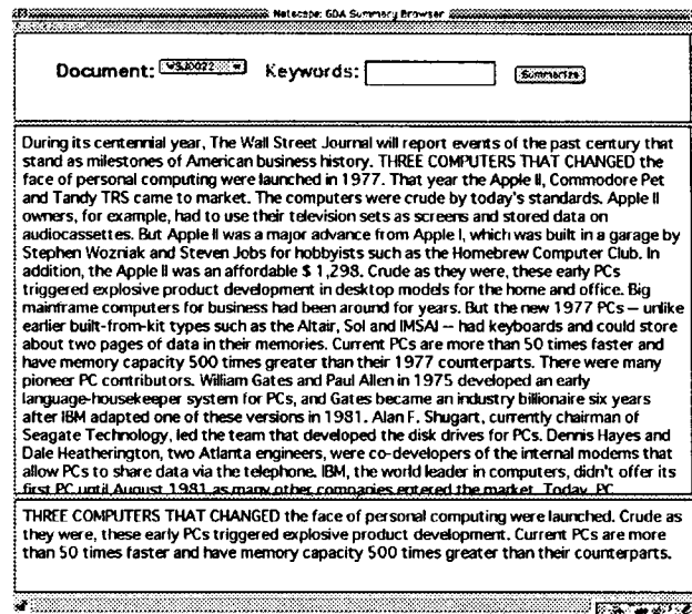
Figure 2: Summary Browser
