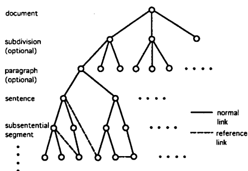
Figure 1: Intra-Document Network
