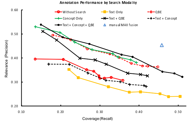
Fig. 4: Search modality comparison. Querying by image and by concept greatly outperforms text search, as text search re-emphasizes the noisy transcript. MAX fusion selects the best performing individual metric for a shot, and outperforms the automatic fusion modalities.
