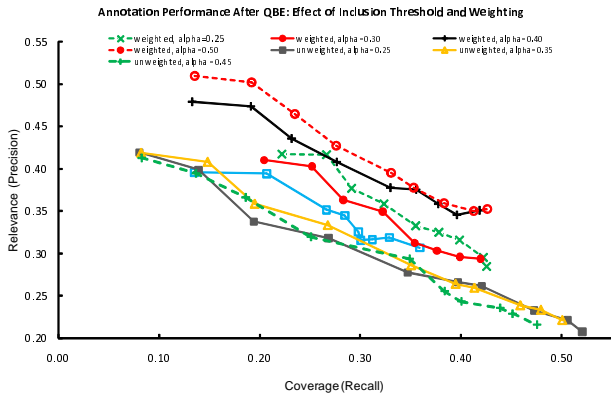
Fig. 5: Performance by inclusion constraint and weighting scheme. Individual runs vary the \alpha parameter in equation (2). Best performances at high \alpha , with fewer included shots. Better performance using weighted similar video inclusion compared to unweighted.
