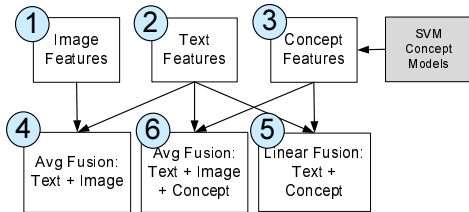
Fig. 2: Diagram of search modalities.
