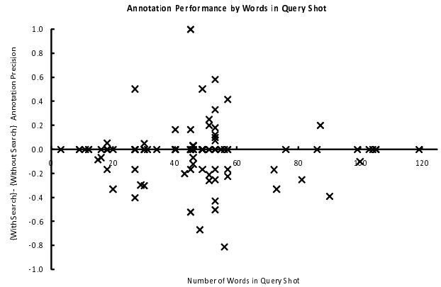
Fig. 6: Difference between annotation extended with text search and without search, using only original transcript, by number of words in query clip. Random scattering shows that successfulness of text-based search does not rely solely on number of words.
