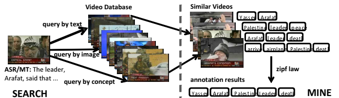
Fig. 1: System diagram. System first collects similar videos using various search algorithms. The ASR/MT transcript of the similar videos are used in a mining step to generate tag annotations for the query video.
