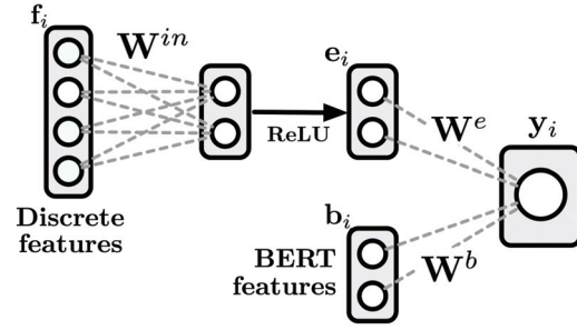
Figure 2: The detection module uses discrete features f_i and BERT embedding b_i to calculate logit y_i .
