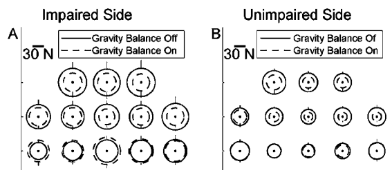
Fig. 4. Mean effect of gravity balance across four subjects. Circle radius is the magnitude of force required to hold the subjects' arms at the test fixture locations shown in Fig. 3. Vertical bars indicate one standard deviation across subjects. (A) Impaired arm. (B) Unimpaired arm.
