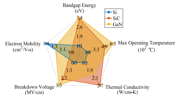
FIGURE 3. Electrical and thermal properties of Si, SiC, and GaN.
