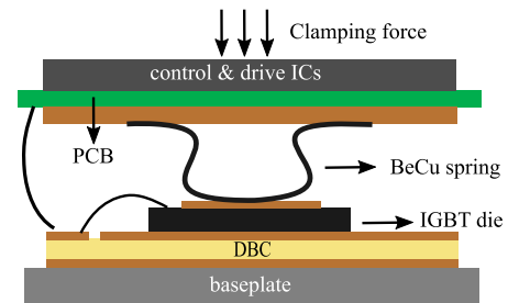
FIGURE 28. Press pack IGBT module with BeCu spring [116].
