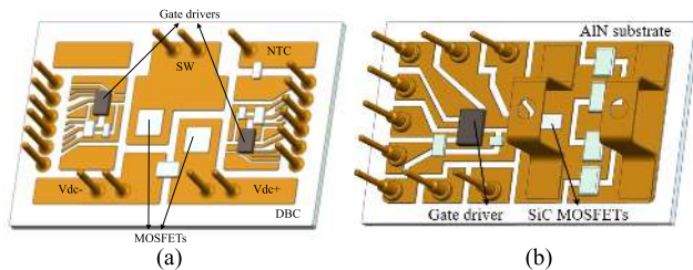
FIGURE 18. DBC based gate driver integrated modules [82], [86].
