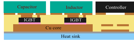
FIGURE 24. HI-LEVEL module for automotive application [103].
