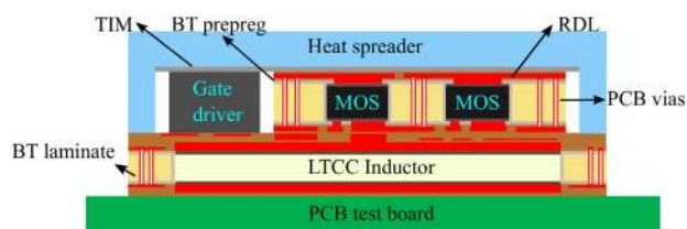
FIGURE 20. PCB Embedded package with LTCC inductor [91].
