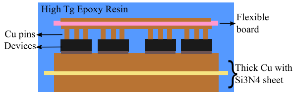
FIGURE 17. Section view of Fuji Electric SiC modules [80].
