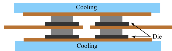
FIGURE 27. Press pack module using Mo pins [99].
