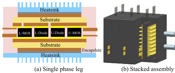
FIGURE 30. Modular double-side cooling 3D packaging [120].
