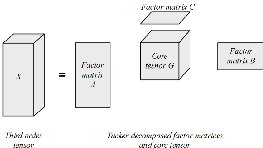
Figure.1 Tucker decomposition of the tensor in the three ways case, the tucker decomposition
