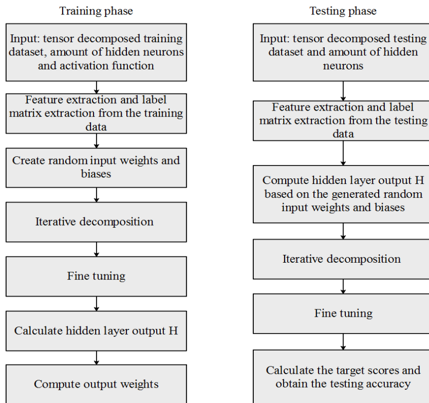
Figure.2 Automotive rank selection based ELM
