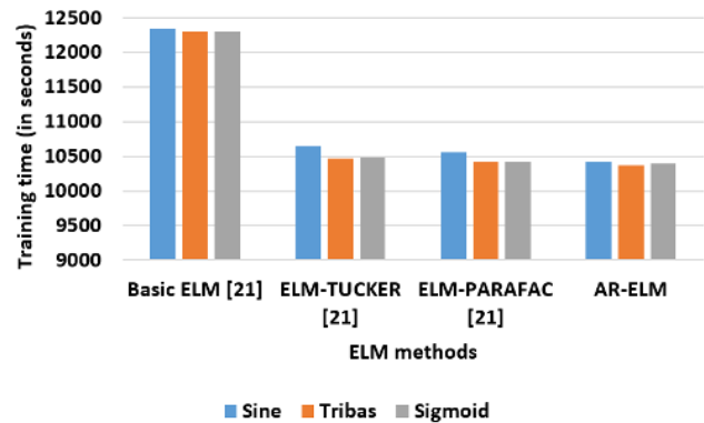
Figure.3 Comparative analysis of training time for MNIST handwritten dataset
