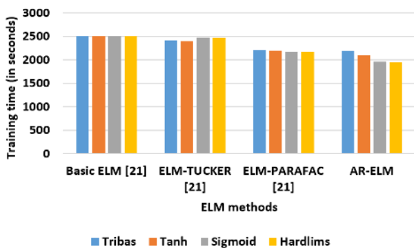
Figure.7 Comparative analysis of training time for Letter Recognition dataset
