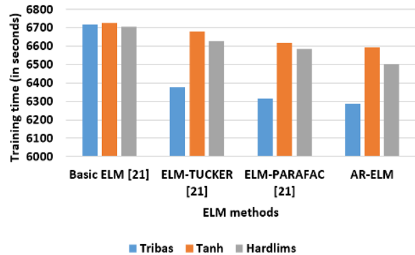
Figure.6 Comparative analysis of training time for shuttle dataset
