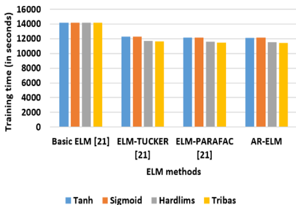
Figure.4 Comparative analysis of training time for KDD Cup 1999 dataset
