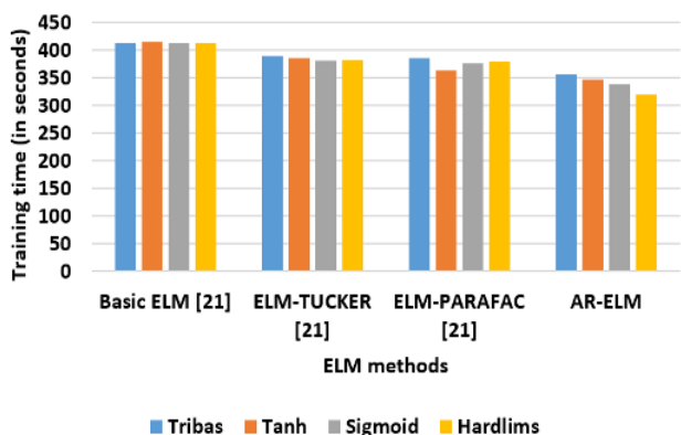
Figure.8 Comparative analysis of training time for Mushroom dataset
