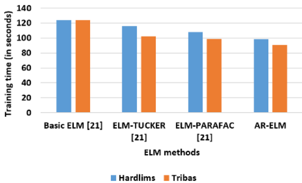
Figure.5 Comparative analysis of training time for satellite dataset
