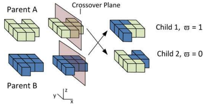
Fig. 6. A crossover operation between two ANT parents. “Compatible” neuron genes are interchanged as shown resulting in two offspring.
