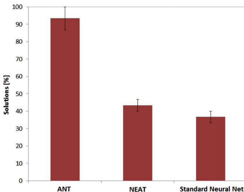
Fig. 11. Probability of finding a solution (fitness \geq 0.9 ) averaged over 30 training runs for ANT, NEAT and standard neural networks.
