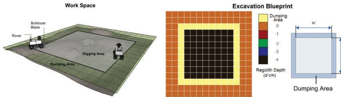
Fig. 7. A typical workspace for the excavation task (left). A corresponding excavation blueprint consisting of an excavation area surrounded by a dumping area (right). The blueprint is compared against the current workspace topology to compute a fitness that ranges from 0 to 1, where 1 corresponds to the desired topology as specified by the blueprint.
