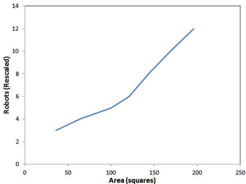
Fig. 20. Excavation performance of ANT solutions evolved using four robots on a 8 × 8 excavation area for varying excavation area.
