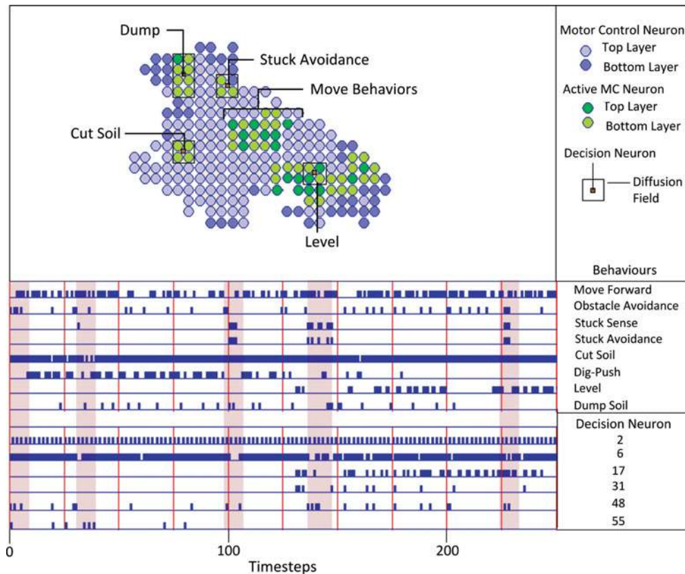
Fig. 14. ANT topology and neuronal activity identifying important behaviors evolved for the excavation task. Shaded columns highlight correlation in neuronal and behavioral activity during a typical simulation run. The controller was evolved using four robots in a 8 \times 8 excavation area and has a fitness of 0.99.
