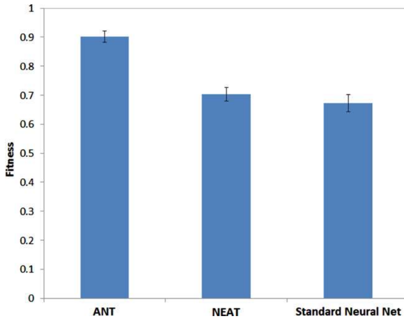
Fig. 10. Maximum fitness averaged over 30 training runs for ANT, NEAT and standard neural networks.
