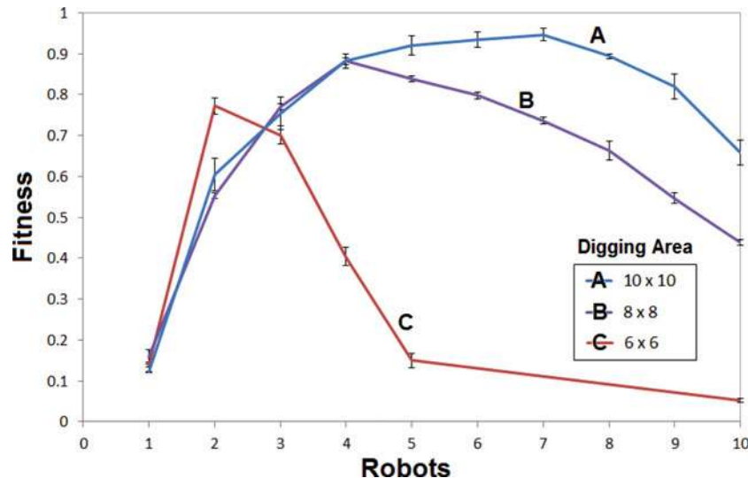
Fig. 18. Excavation performance ANT-based solutions evolved using four robots ( 8 \times 8 excavation area) applied to resized excavation area and the number of robots.
