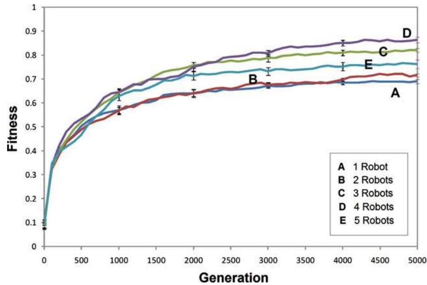
Fig. 9. Fitness comparison of ANT-based solutions during training for between 1 and 5 robots averaged over 30 runs.
