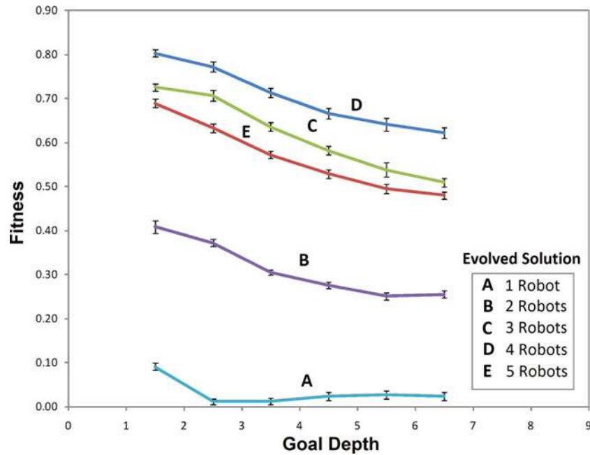
Fig. 21. Excavation performance of ANT-based solutions for varying depth taken after 10,000 timesteps.
