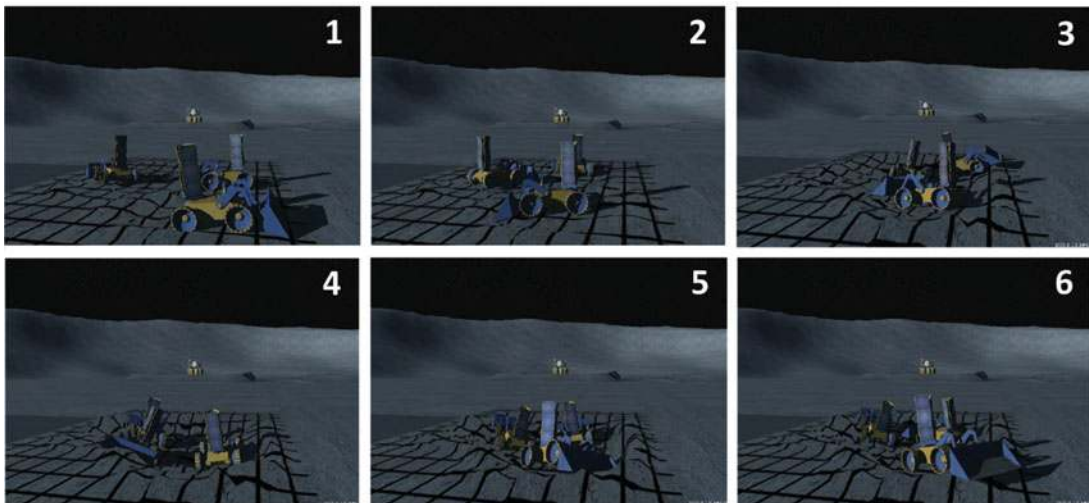
Fig. 25. Digital Spaces™ simulation of three robots using a four-robot ANT controller solution to perform excavation on simulated lunar terrain. The robots unlike under training conditions use a front-loader bucket instead of a two-way bulldozer blade. The excavation blueprint includes a hole and a ramp for the robot to enter/exit surrounded by the dumping area.
