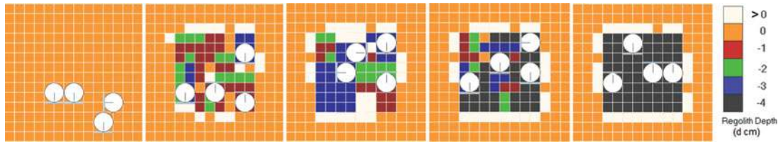
Fig. 15. Simulation snapshots of an excavation task simulation (four robots) after 0, 50, 75, 100, 170 timesteps.
