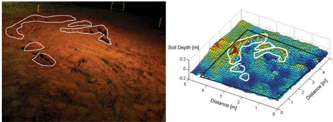
Fig. 30. Photo of the work site after excavation (left). Mounds of dirt (berms) highlighted. 3D laser scan of work site with berms highlighted (right).
