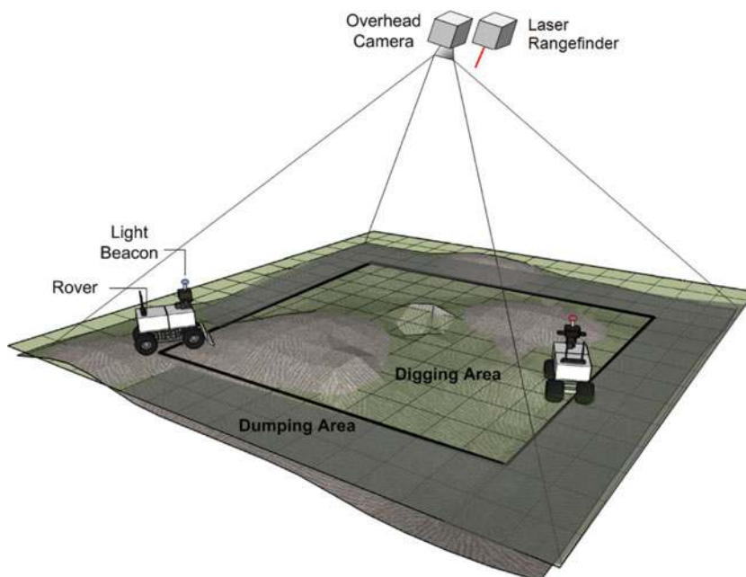
Fig. 27. Layout of the experimental system, showing excavation robots mounted with light beacons localized using an overhead camera system.
