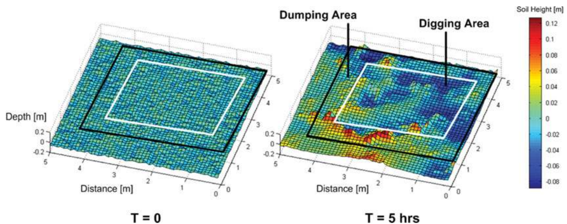
Fig. 29. An overhead laser scan showing the difference in soil height before and after the excavation experiment.
