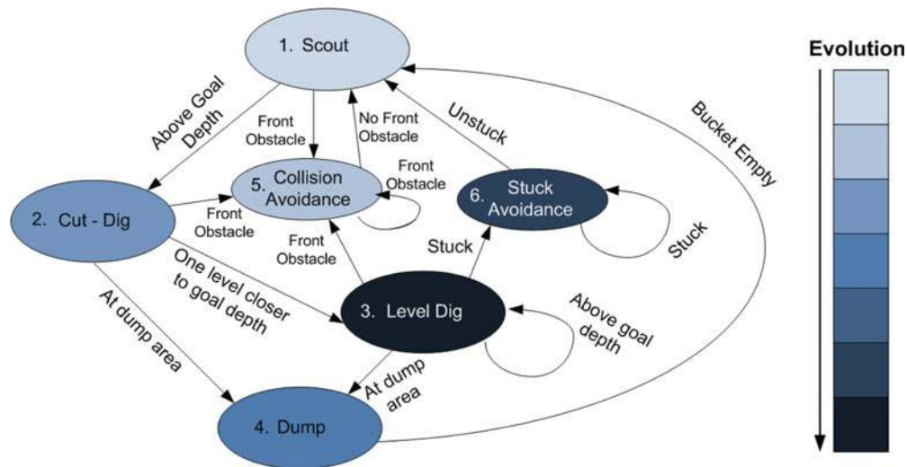
Fig. 16. Representation of major behavior states evolved by the ANT solution controllers. Shading indicates the order in which these complex behaviors are evolved.
