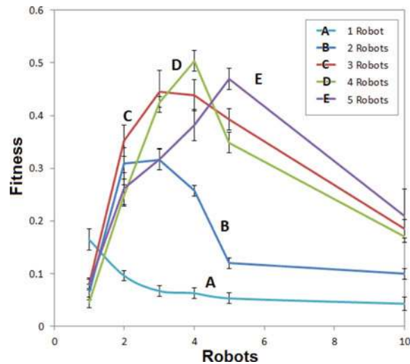
Fig. 19. Excavation performance of the fittest standard neural networks evolved using between 1 and 5 robots applied to scenarios using 1–10 robots.
