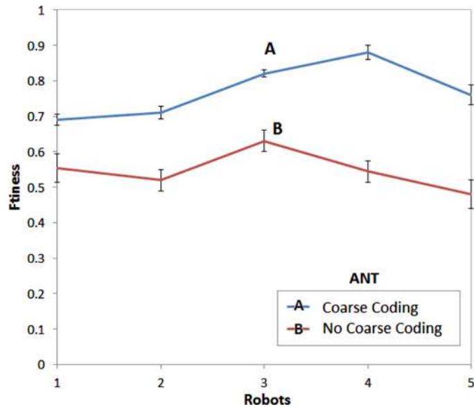
Fig. 12. Maximum fitness of ANT with and without-coarse coding for between 1 and 5 robots.
