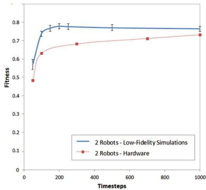
Fig. 28. Fitness during a typical excavation run of an ANT controller evolved using four robots ( 8 \times 8 area) applied to two robots on the training simulator and real robots.
