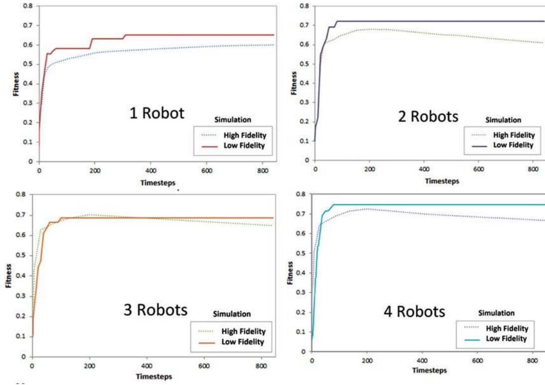
Fig. 24. Fitness comparison of ANT controllers in the low-fidelity training simulator and high-fidelity Digital Spaces™ simulator.
