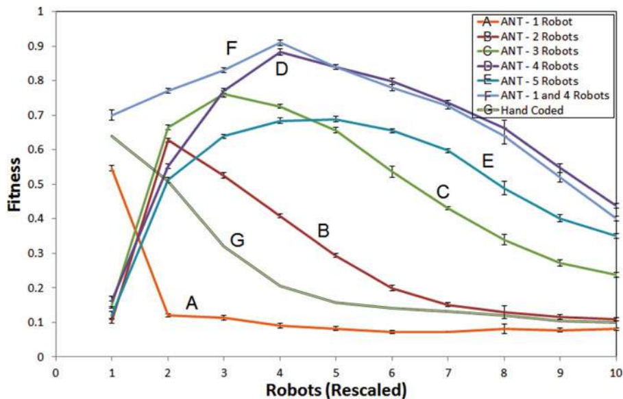
Fig. 17. Excavation performance of ANT-based solutions evolved using 1–5 robots ( 8 \times 8 excavation area) applied to scenarios using 1–10 robots.
