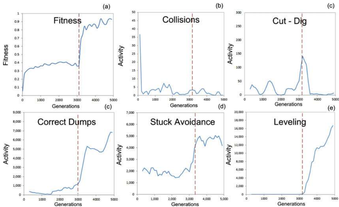
Fig. 13. (a) Fitness. (b)–(f) Evolution of important behaviors for the excavation task during a typical evolutionary training run of ANT. At generation, 3100 new behaviors are discovered foreshadowing a rapid rise in fitness and convergence to a solution.
