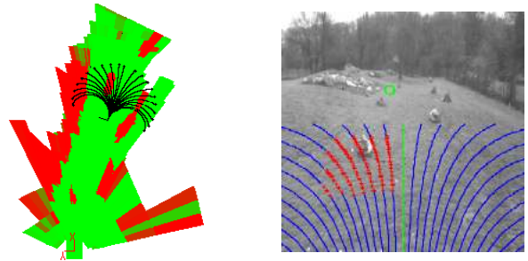
Figure 6: A set of circle arcs to evaluate on the global probabilistic model (left), and reprojected in the current camera view (right)
