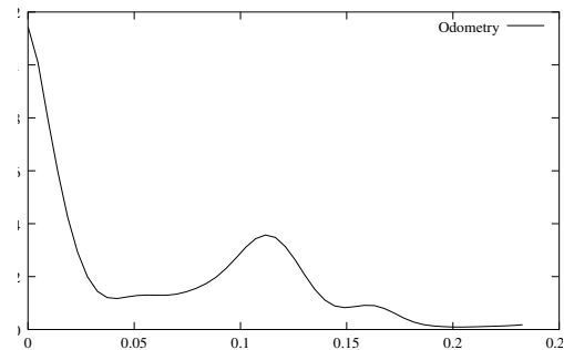
Figure 10: Histogram of odometry errors measured every 0.5m steps during a 50 meter run with Lama on various kinds of ground.
