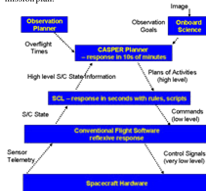
Figure 2: Autonomy Software Architecture
