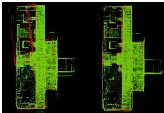
Fig. 6: Map created by Au-Spot exploring Eagle Rock Substation, with different odometry sources: proposed method in green against KO in red (left) and KVO in red (right).
