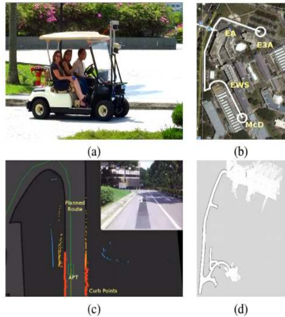
Fig. 4 Autonomous system demonstration. (a) Vehicle in operation, (b) Pickup-Dropoff points, (c) Snapshot of curb localization estimate, (d) curb map augmented by planar patches (25) .
