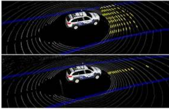
Fig. 6 Road marking detection through histogram thresholding. Blue lines are the road bounds estimated by curb detector and yellow points correspond to the detected road marking (Top: crosswalk; Bottom: double line) (15) .
