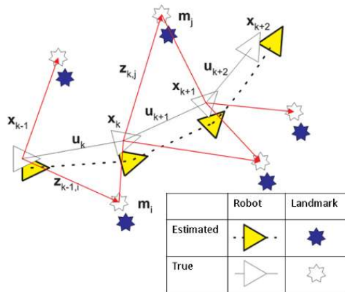
Fig. 3 Demonstration of SLAM problem (17) .
