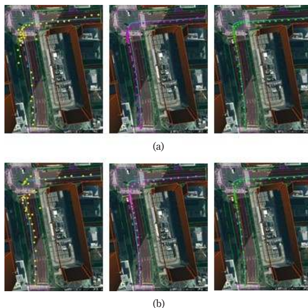
Fig. 14 Visualization of results: GNSS result (yellow dot), GNSS/INS integration result (purple dot), and GNSS/INS/lane detection integration result (green dot). (a) First right turning experiment. (b) Second right turning experiment.
