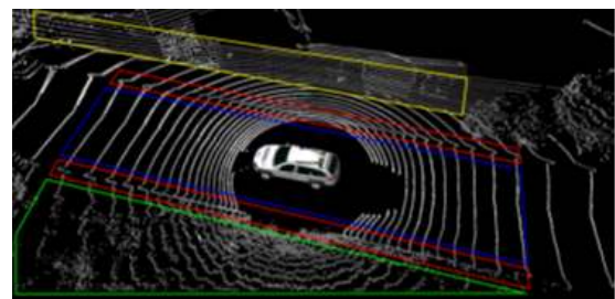
Fig. 5 Laser ring compression level is related to the surface slope. In this frame obstacles can be roughly distinguished as walls (yellow field), grass (green field), road (blue field) and curbs (red field). They are estimated using the ring compression data (14) .
