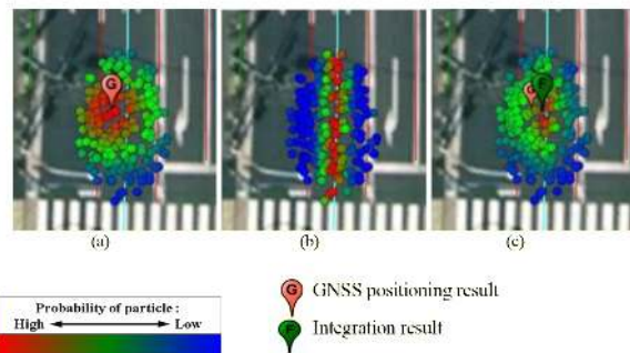
Fig. 13. Demonstration of probability evaluation for particles.
