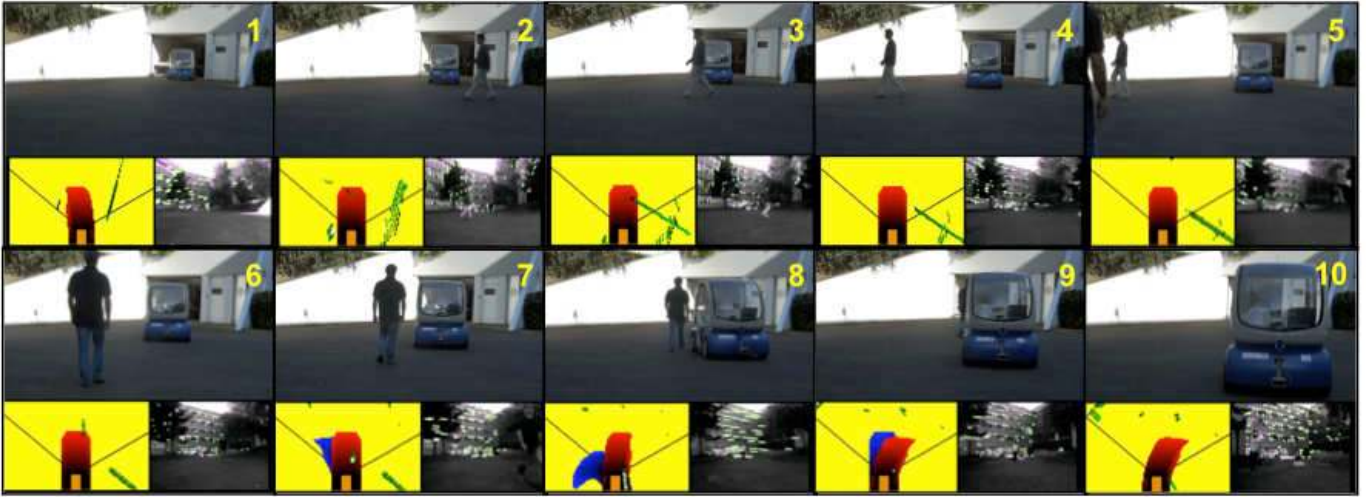
Fig. 3. Ten relevant iterations of the experiment with two crossing pedestrians. For each iteration, we show the occupancy grid (left) and current image (right). In the occupancy grid, the dangerous cell sets associated with the visual tentacle and to the best tentacle (when different) are shown, and two black segments indicate the lidar amplitude. Only cells that we predict to be occupied in the next T s have been drawn in the grid. The segments link the current and next key image points.
