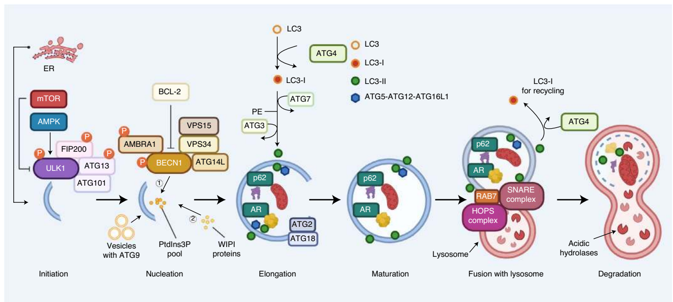
Fig. 2 | Core machinery of autophagy. Initiation of autophagy requires the ULK1 kinase complex, which is tightly regulated by AMPK and mTOR, which act as an activator and inhibitor, respectively. AMPK activates ULK1 through phosphorylation. The ULK1 complex, composed of FIP200, ATG13 and ATG101, stimulates the class III phosphatidylinositol 3-kinase (PIK3C3) complex, which is composed of BECN1 (which can be inhibited by BCL-2), AMBRA1, ATG14L, VPS15 and VPS34. This complex then produces a pool of phosphatidylinositol 3-phosphate (PtdIns3P), which leads to the recruitment of WIPI proteins, which recover ATG9-positive vesicles from previous membranes, as well as recruiting the ATG5-ATG12-ATG16L1 (E3) complex. LC3 is first cleaved by the ATG4 protease to form cytosolic LC3-I, which is further recognized by E1 (ATG7), E2 (ATG3) and E3 components, leading to its conjugation to phosphatidylethanolamine (PE). After this process, LC3-I is referred to as LC3-II. LC3-II binds to LIR-containing autophagy receptors (AR; such as p62) bound to cargo targeted for degradation. Fusion of autophagosomes with lysosomes is mainly mediated by the assistance of RAB proteins, SNARE proteins and a HOPS complex. After fusion, the cargo is degraded by lysosomal hydrolases and the degradation products can be reused by the cell. LC3-II bound to the outer membrane is cleaved by ATG4 to be reused for a new round of lipidation.
