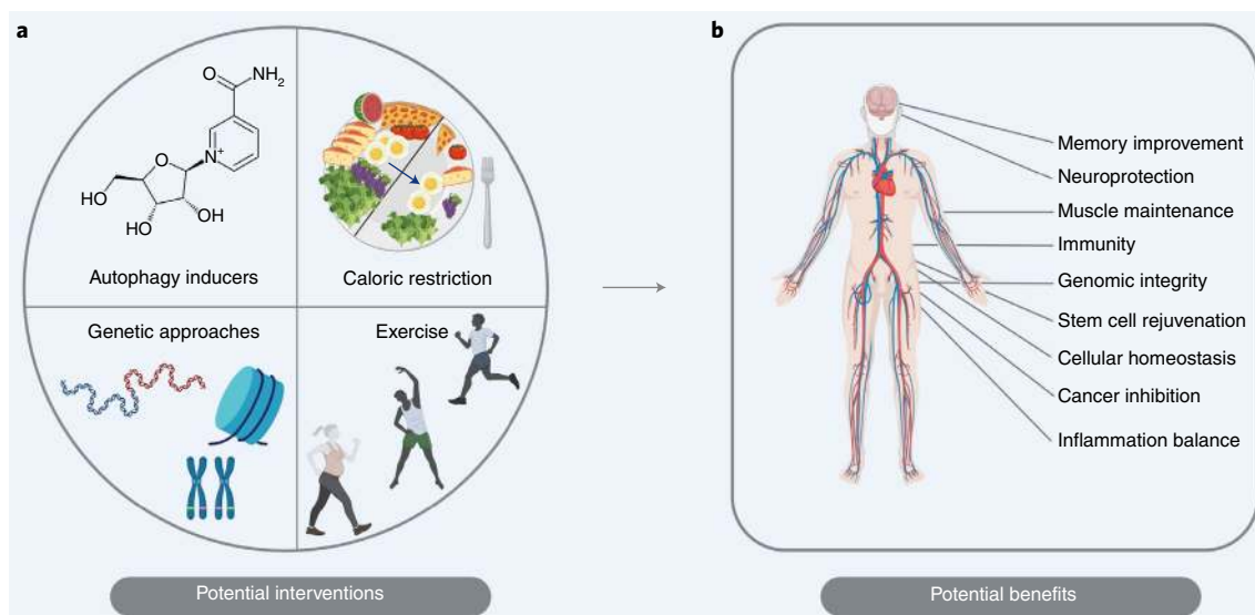
Fig. 4 | Maintaining autophagy through lifestyle and medical interventions prolongs longevity. a , Potential interventions to stimulate autophagy: autophagy inducers, dietary restriction, exercise and genetic approaches. b , Autophagy induction could positively impact human health.
