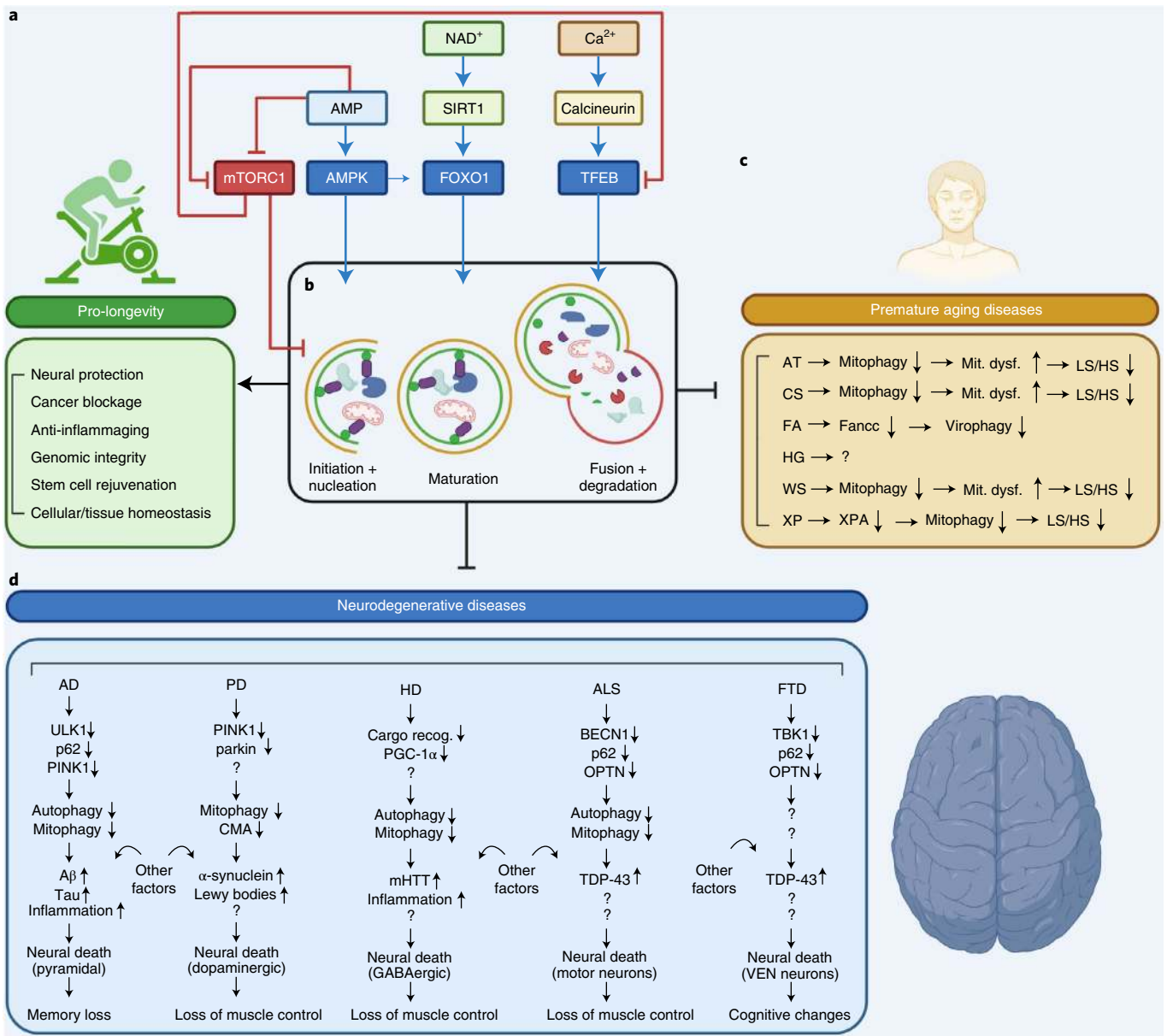
Fig. 3 | Autophagy in health and disease. a , Autophagy participates in multiple processes that are essential for longevity. b , A brief summary of some of the major known mechanisms that regulate autophagy in multiple organisms and their influence on the process. c , A list summarizing premature aging diseases with impaired mitophagy as a cause of mitochondrial dysfunction, which contributes to short lifespan (LS) and healthspan (HS). These premature aging diseases are ataxia telangiectasia (AT), Cockayne syndrome (CS), Fanconi anemia (FA), Hutchinson–Gilford syndrome (HG), Werner syndrome (WS) and xeroderma pigmentosum (XP; especially group A). Changes in autophagy and mitophagy in Hutchinson–Gilford syndrome are elusive. d , Autophagy (including subtypes of selective autophagy, such as mitophagy) is impaired in broad neurodegenerative diseases, where impairment may drive or exacerbate disease progression. These diseases include AD, Parkinson’s disease (PD), Huntington’s disease, ALS and frontotemporal dementia (FTD). We emphasize that these are not the only drivers of the diseases and other processes may have roles leading to pathology and symptomatology.
