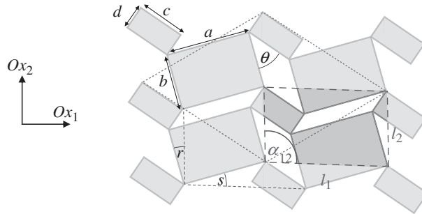
Figure 1. The system made from connected different-sized rectangles of dimensions a \times b and c \times d (denoted by [a \times b, c \times d] ) discussed in this paper. Note that this system may be described in terms of two unit cells (UC1 and UC2) and in the derivation presented here, the system is aligned in the Ox_1 – Ox_2 plane in such a way that the side of the unit cell UC2 of length l_2 is always parallel to the Ox_2 direction. Grey dashed lines, UC1 and long dashed lines, UC2.
