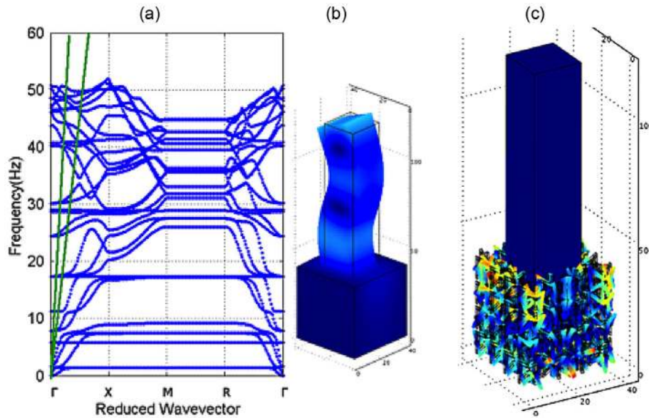
Figure 3. (a) Band diagram for a concrete building ( 20\text{ m} \times 20\text{ m} \times 80\text{ m} ) atop a concrete homogeneous plate ( 40\text{ m} \times 40\text{ m} \times 40\text{ m} ); Floquet-Bloch conditions are set on vertical sides of the plate and stress-free conditions hold elsewhere; Flat bands correspond to eigenmodes of the building around 1 Hz, 9 Hz, 17 Hz, etc. that couple to the flexural band (lowest band at \Gamma ). (b) Representative eigenmode of (a) at 17 Hz. (c) Eigenmode with suppressed building's vibration around 17 Hz when the plate is structured with auxetic metamaterial ( 4^3 elementary cells with bars making an angle as in Figure 2c).
