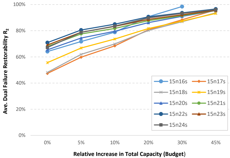
Figure 5.16 – Achievable R 2 vs. Percentage of spare capacity increase on the 15n30s1 network family
